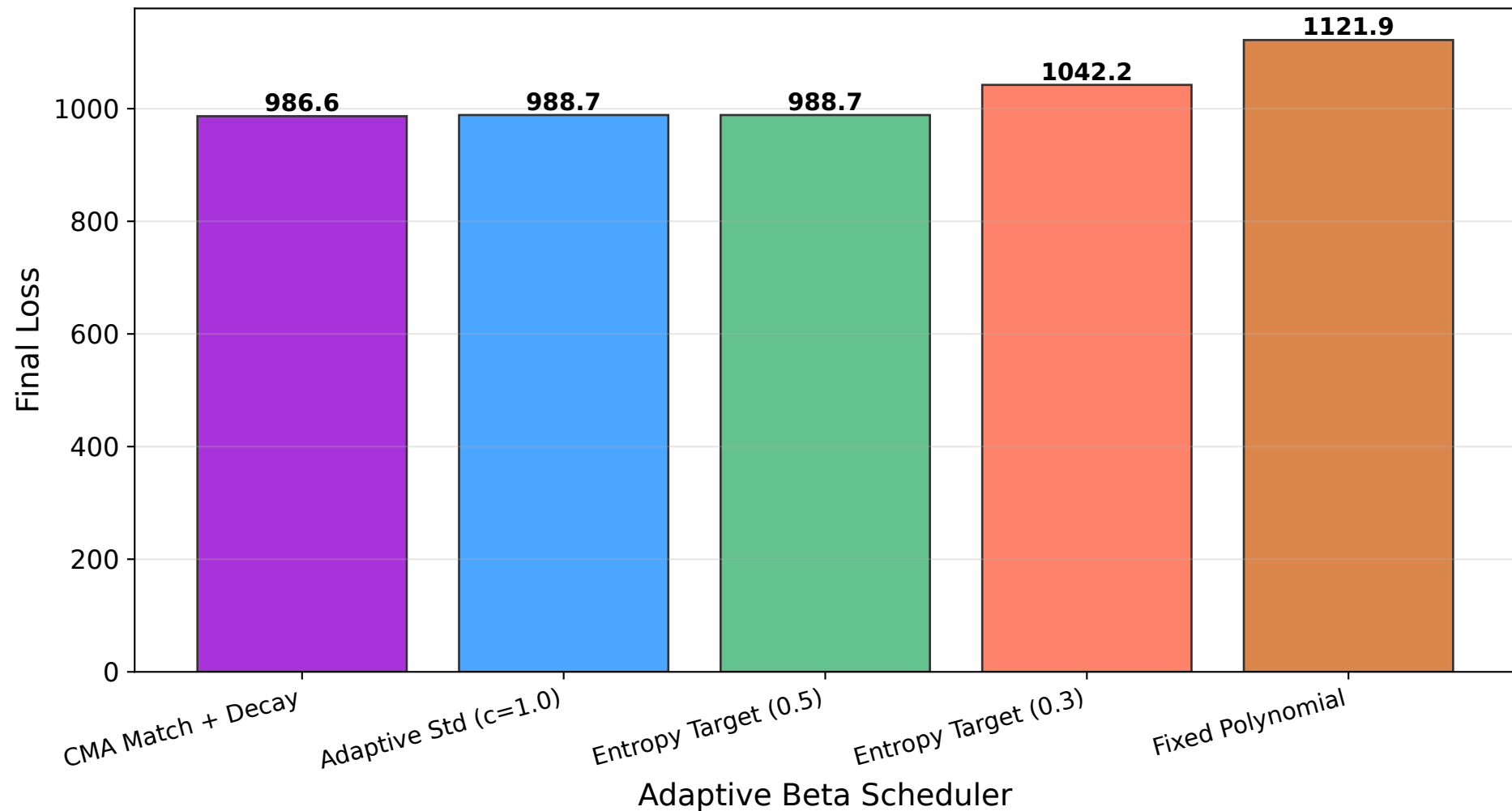
Rosenbrock - Scheduler Performance Comparison (d=1000, K=10, 10000 iterations)
