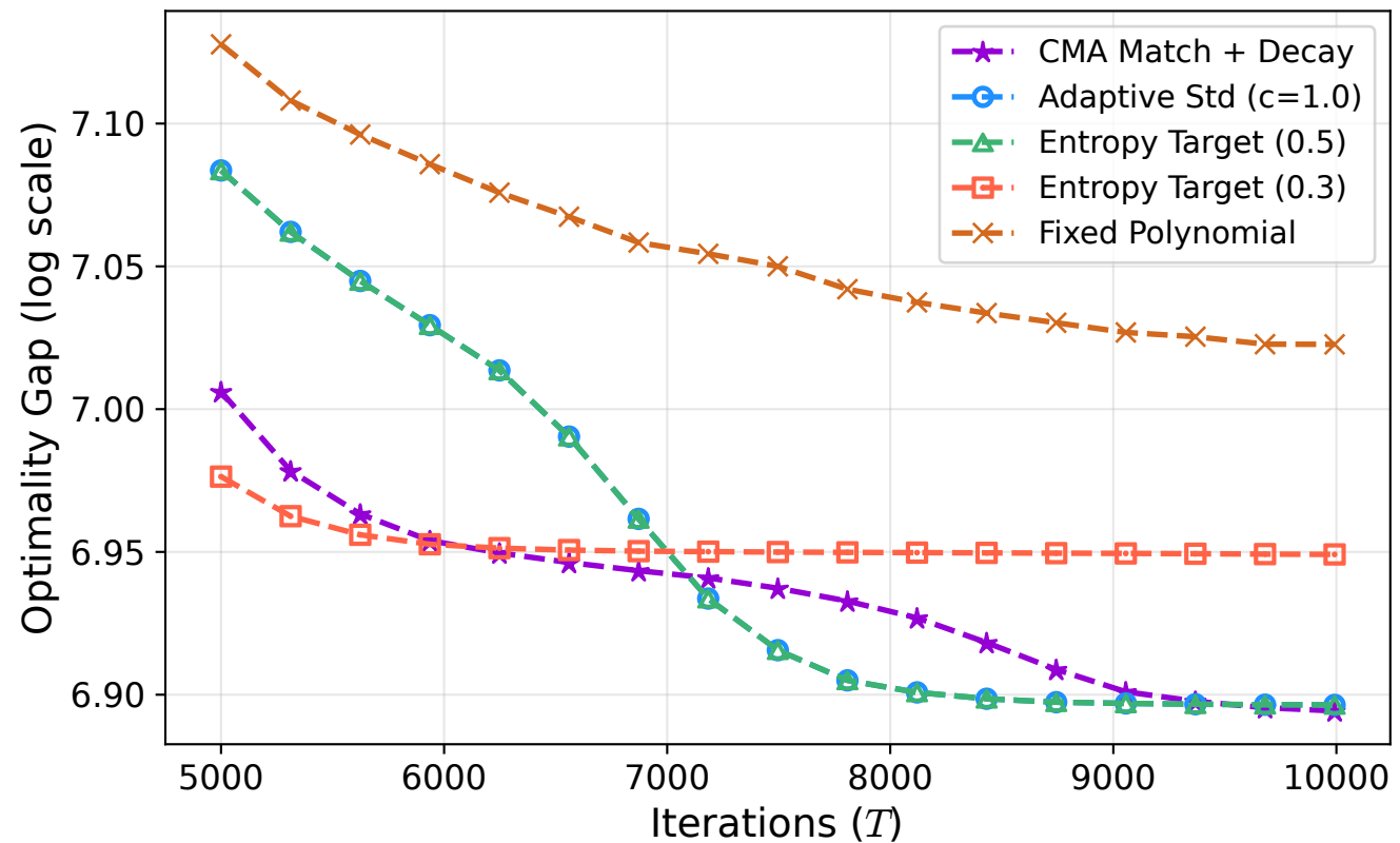
Convergence Phase (Zoomed) (Last 5000 iterations)
