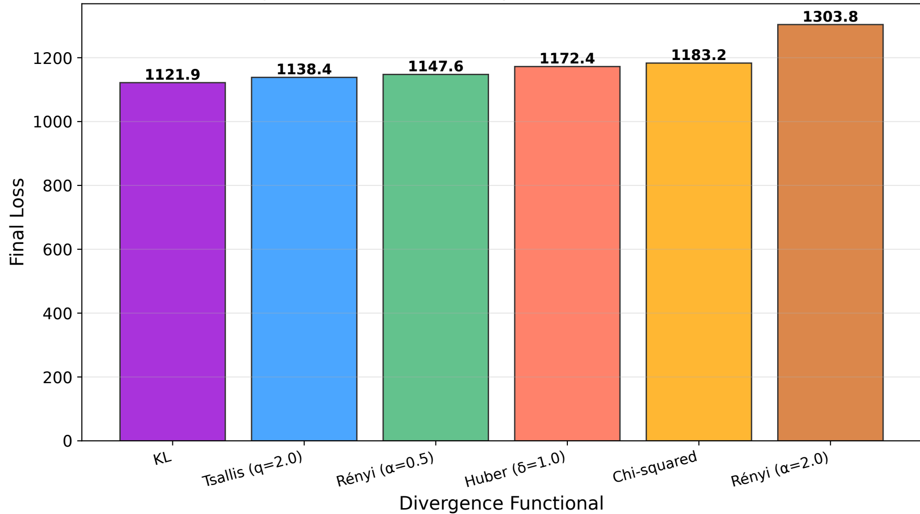
Rosenbrock - Divergence Performance Comparison\n(d=1000, K=10, 10000 iterations)
