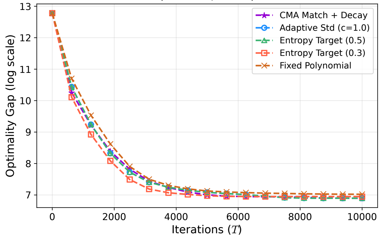
Rosenbrock - Adaptive Scheduler Comparison ( d=1000 , K=10 )
