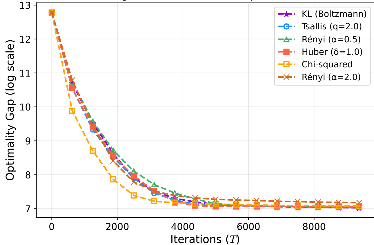
Rosenbrock - Divergence Functional Comparison (d=1000, K=10)
