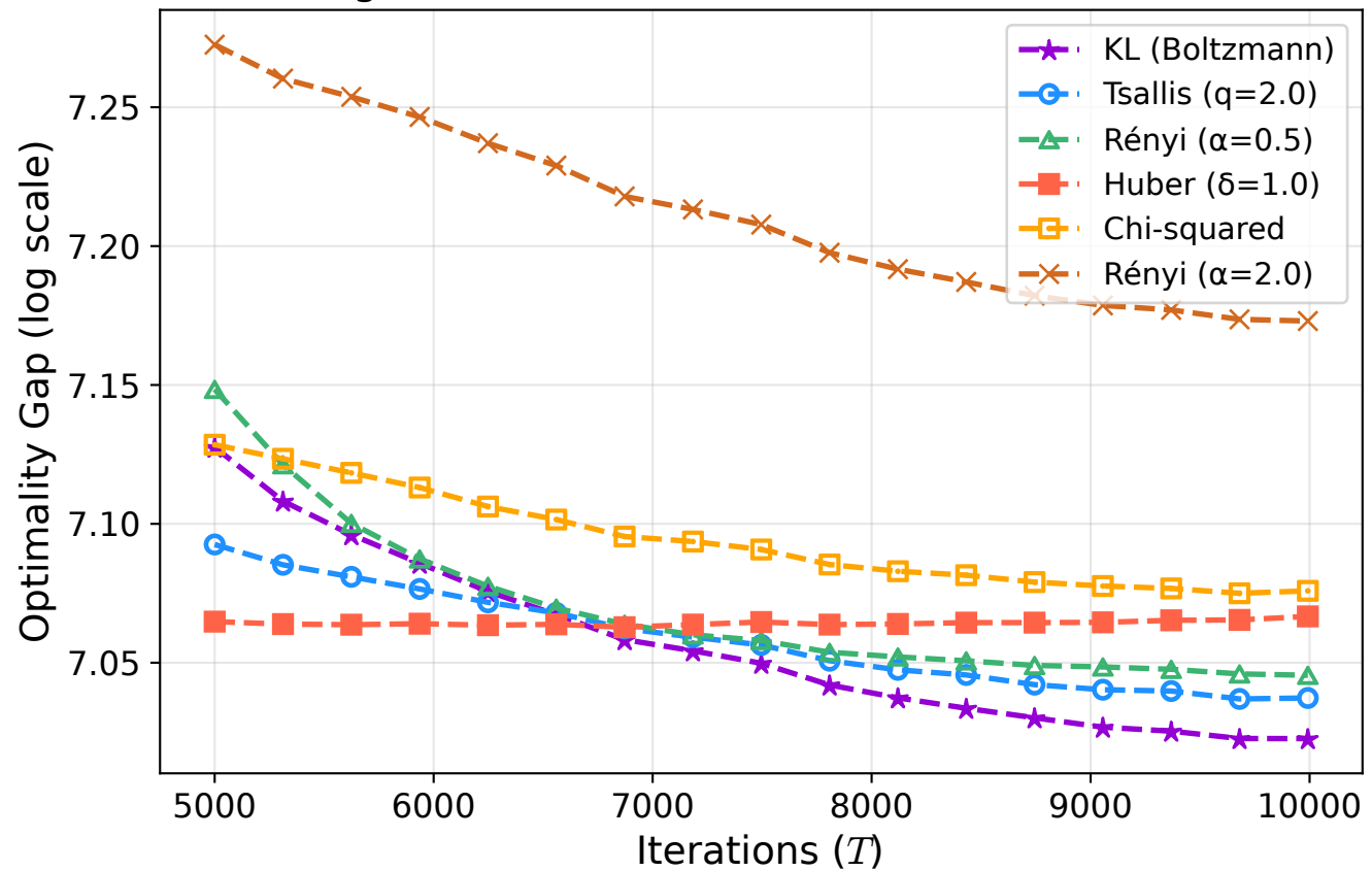
Convergence Phase (Zoomed) (Last 5000 iterations)
