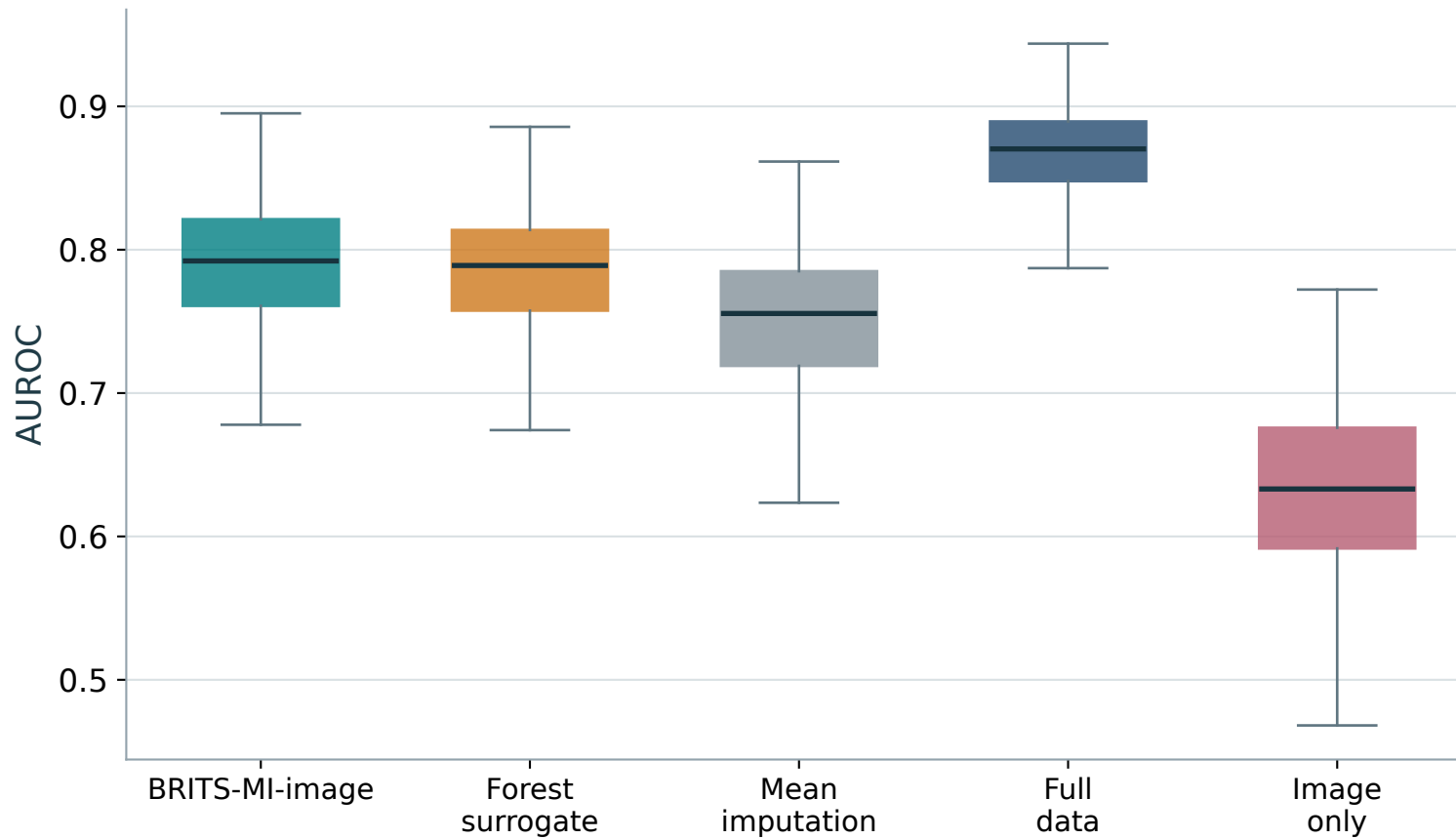
A AUROC Higher is better
