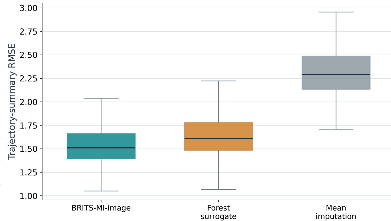
D Trajectory-summary RMSE Lower is better
