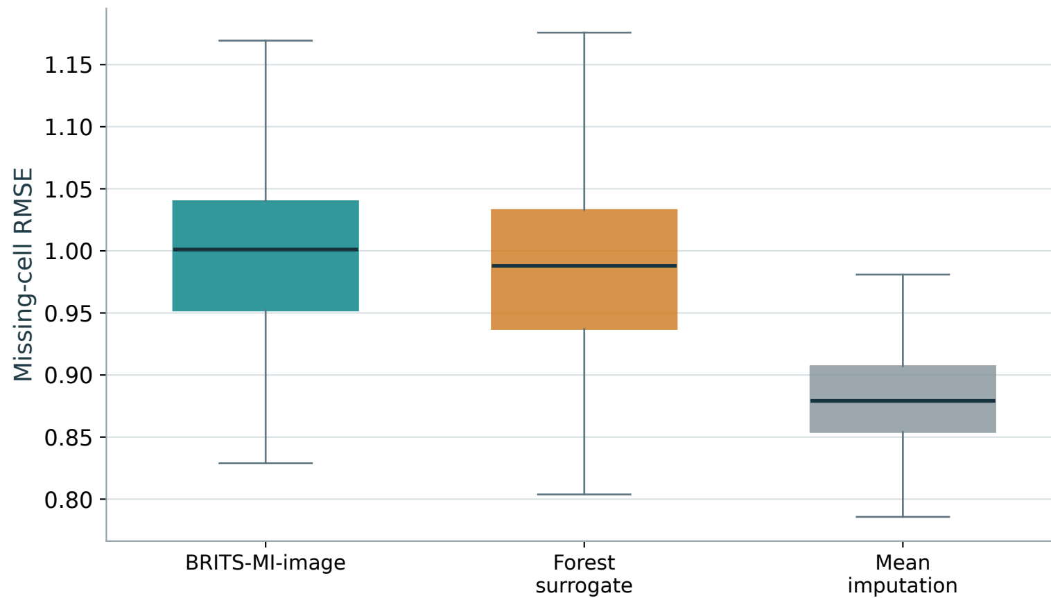
C Missing-cell RMSE Lower is better
