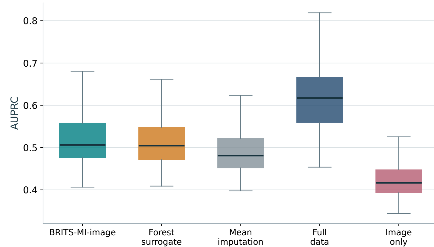
B AUPRC Higher is better
