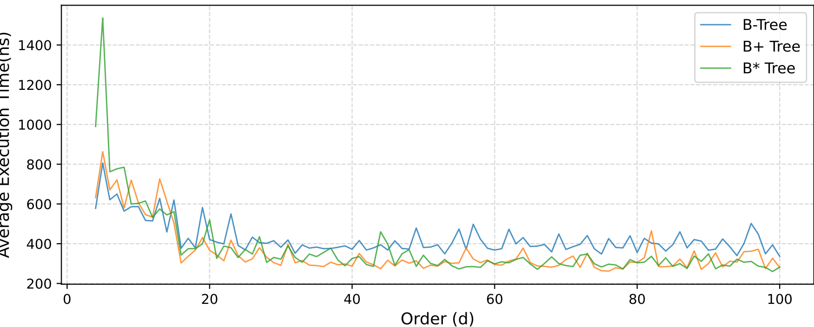
Deletion Execution Time (d = 3 to 100)
