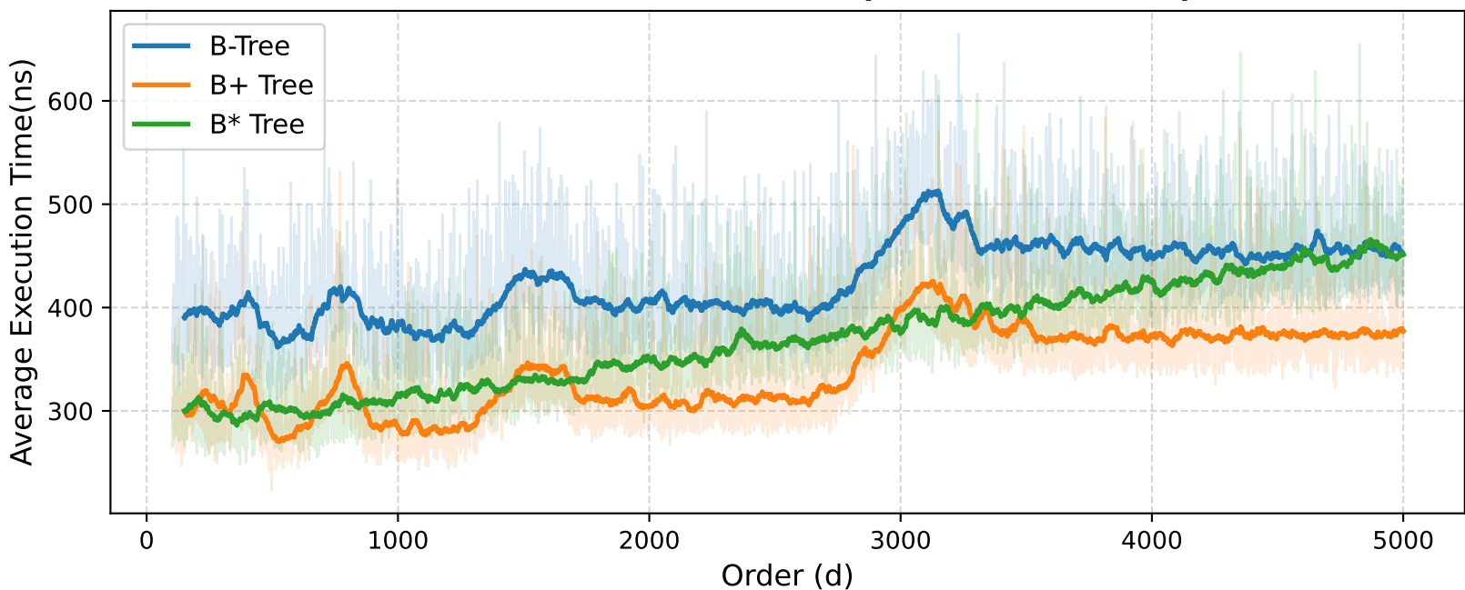
Deletion Execution Time (d = 100 to 5000)
