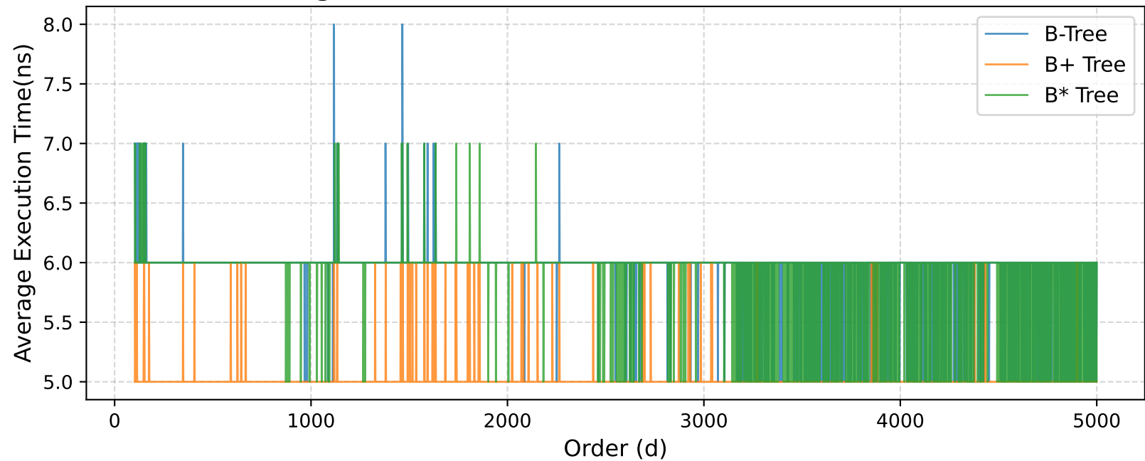
Range Search Execution Time (d = 100 to 5000)
