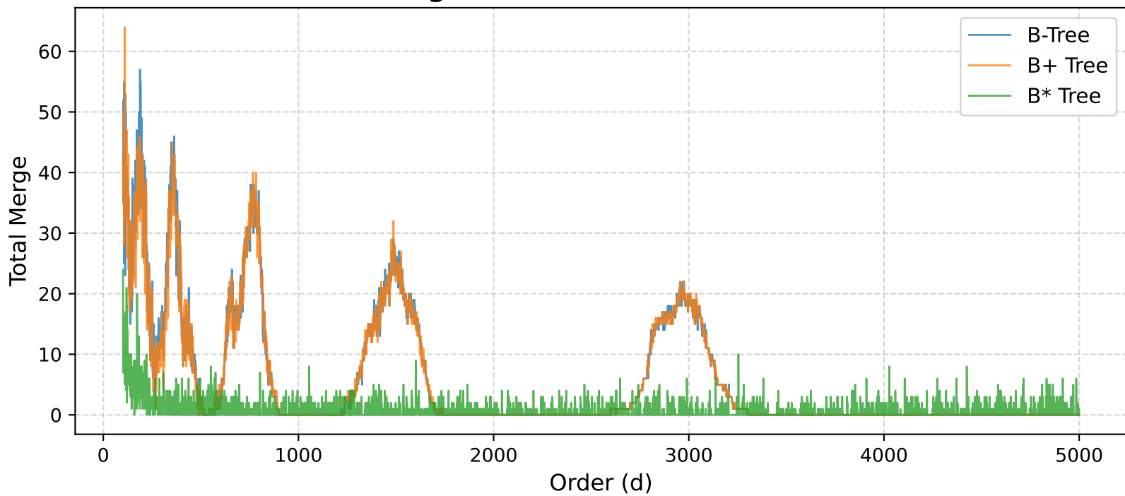
Merge Count (d = 100 to 5000)
