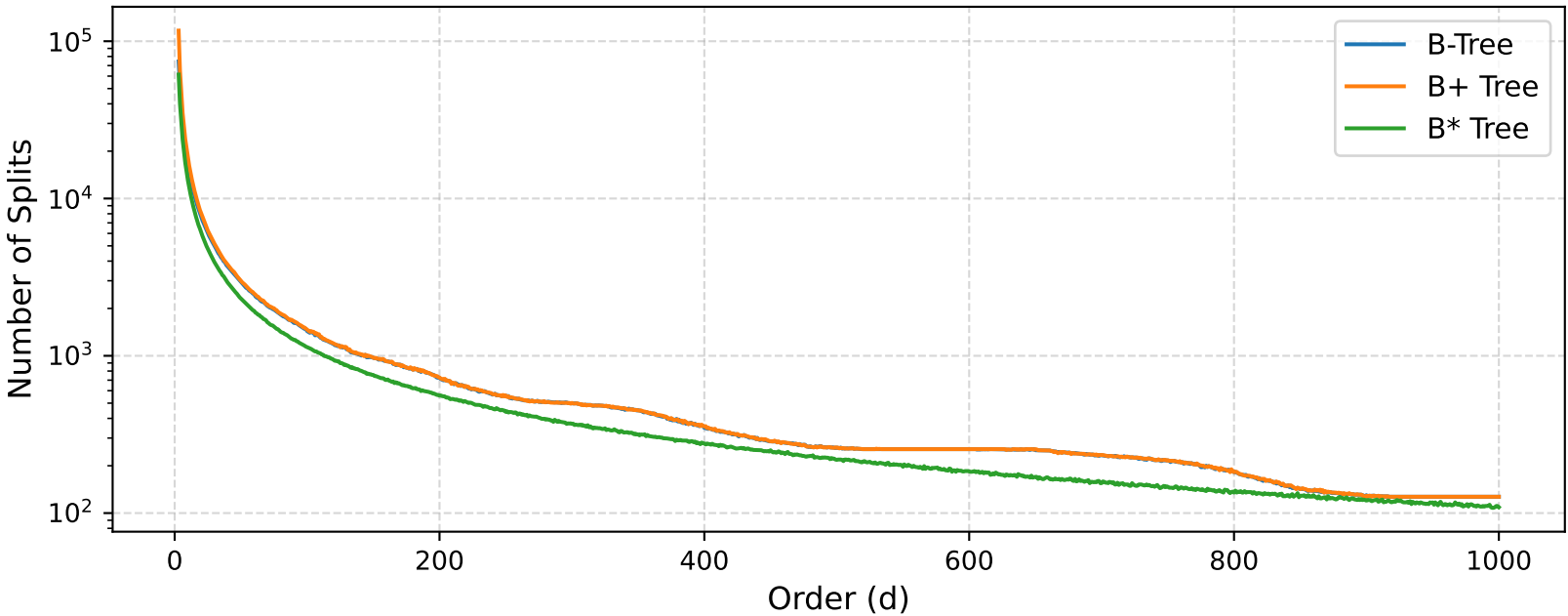
Total Split Counts(Log Scale)
