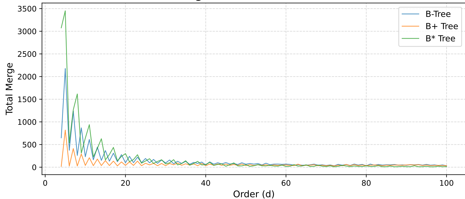
Merge Count (d = 3 to 100)
