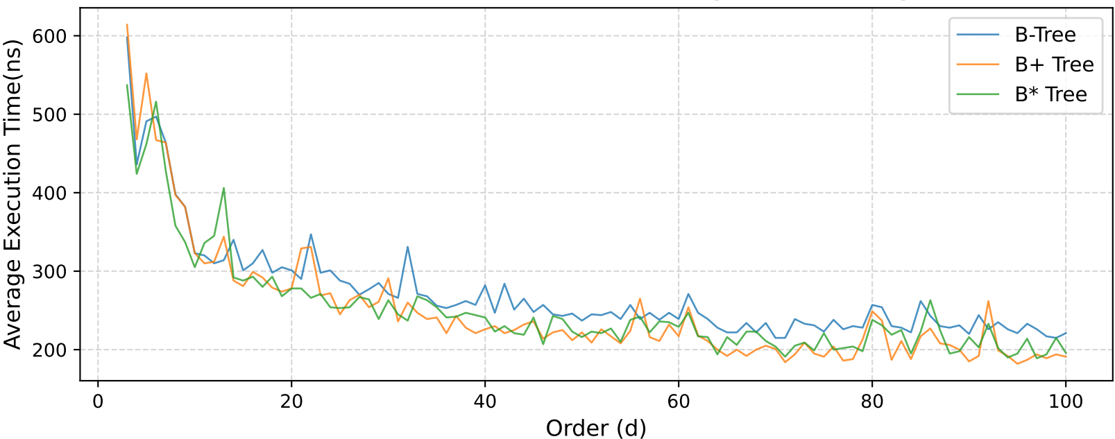
Point Search Execution Time (d = 3 to 100)
