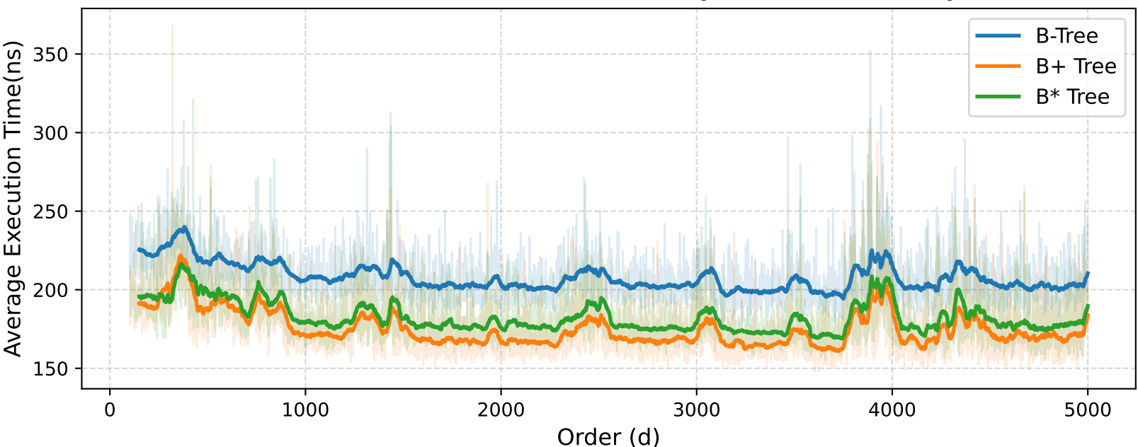
Point Search Execution Time (d = 100 to 5000)
