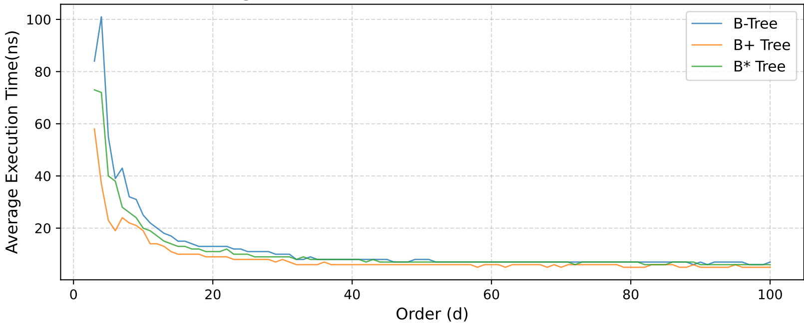
Range Search Execution Time (d = 3 to 100)
