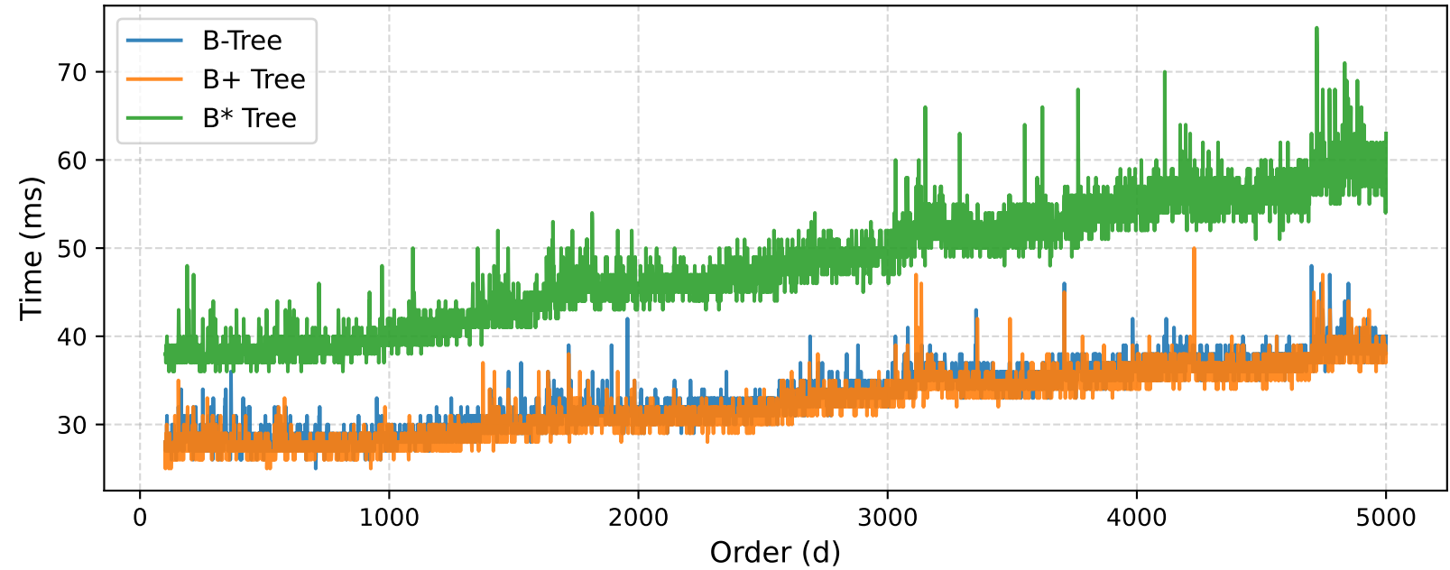
Insertion Time (d = 100 to 5000)
