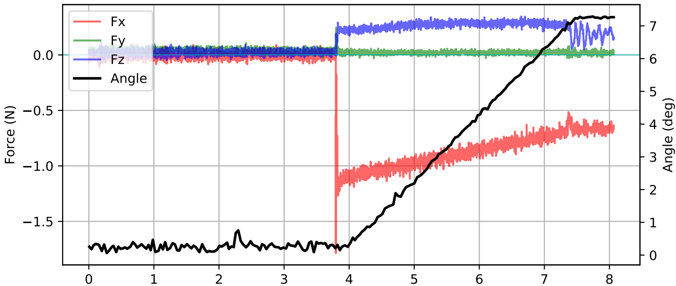
Fit: m=0.64\text{kg} , z_c=0.146\text{m}
