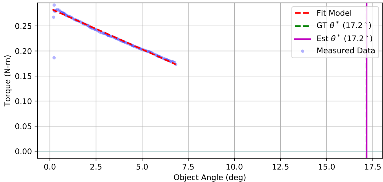
Fit: m=0.64\text{kg} , z_c=0.146\text{m}
