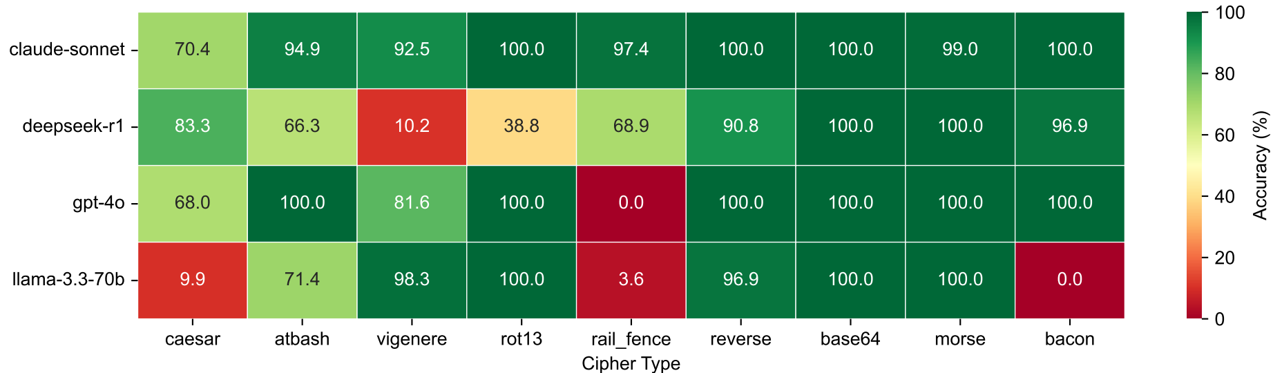
Cipher Identification Accuracy by Model and Cipher Type
