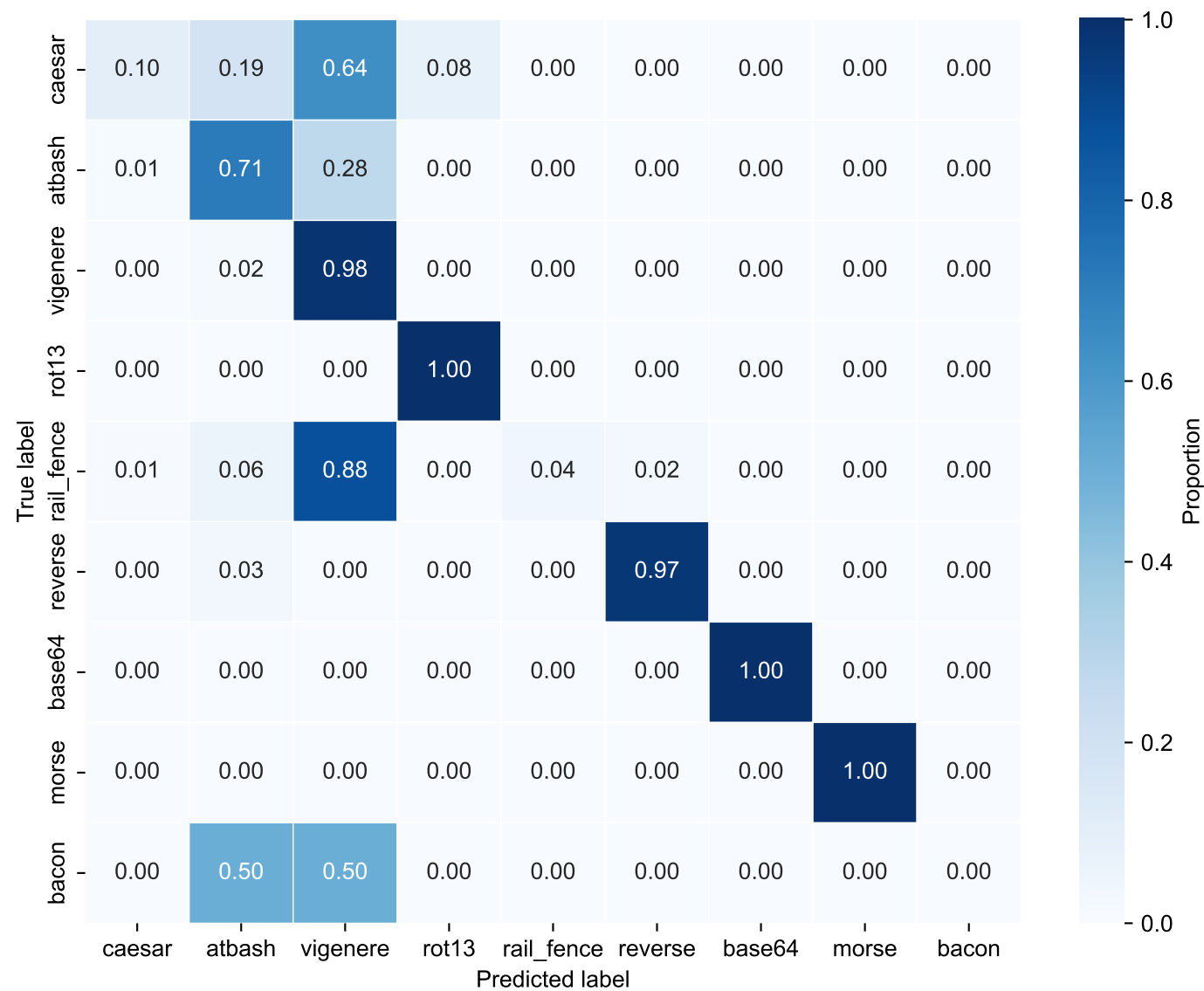
Confusion Matrix — llama-3.3-70b (row-normalized)
