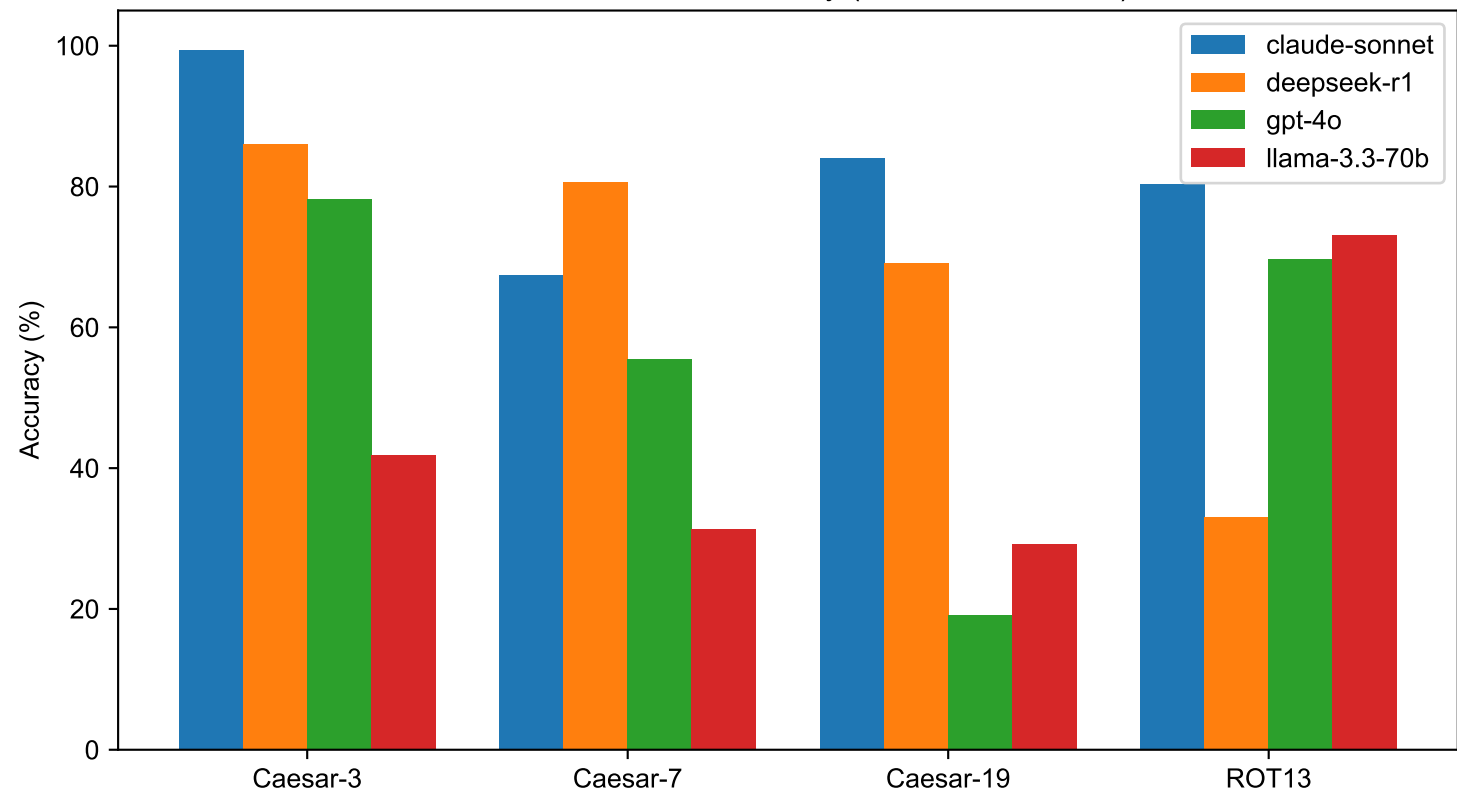
ROT13 vs Caesar Accuracy (Memorization Test)
