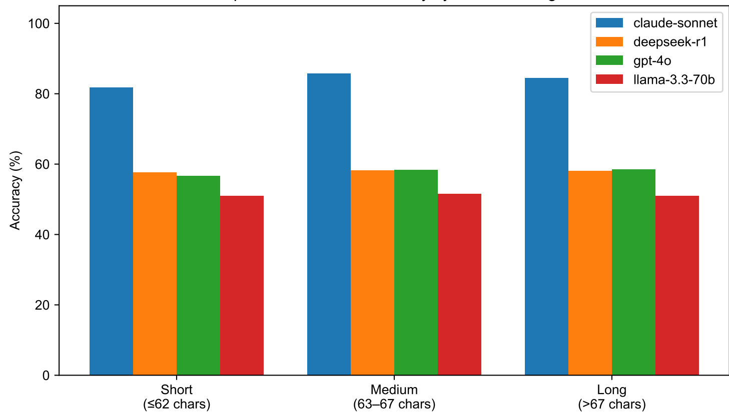
Cipher Identification Accuracy by Plaintext Length
