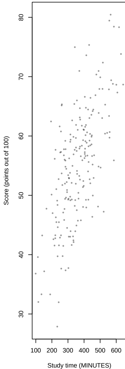
Cov = 729.4
