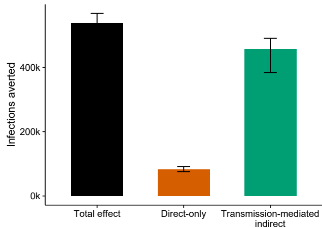
Effect decomposition
