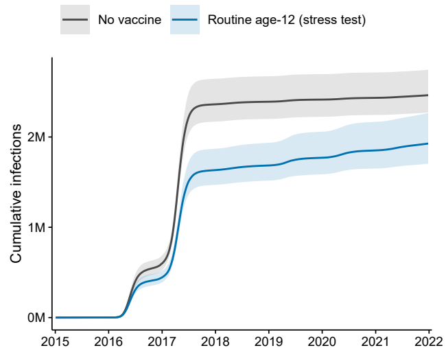
Effect decomposition
