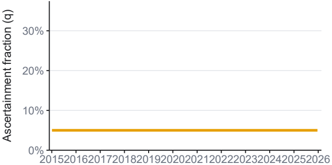
E Case ascertainment q FIXED at 0.05 (not estimated)
