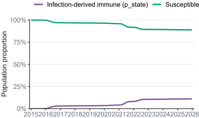
E Case ascertainment q FIXED at 0.05 (not estimated)
