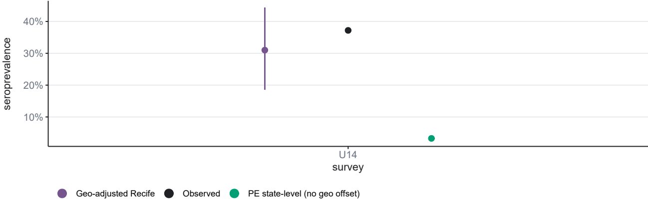
G U14 Recife serosurvey: observed vs model (fixed q)
