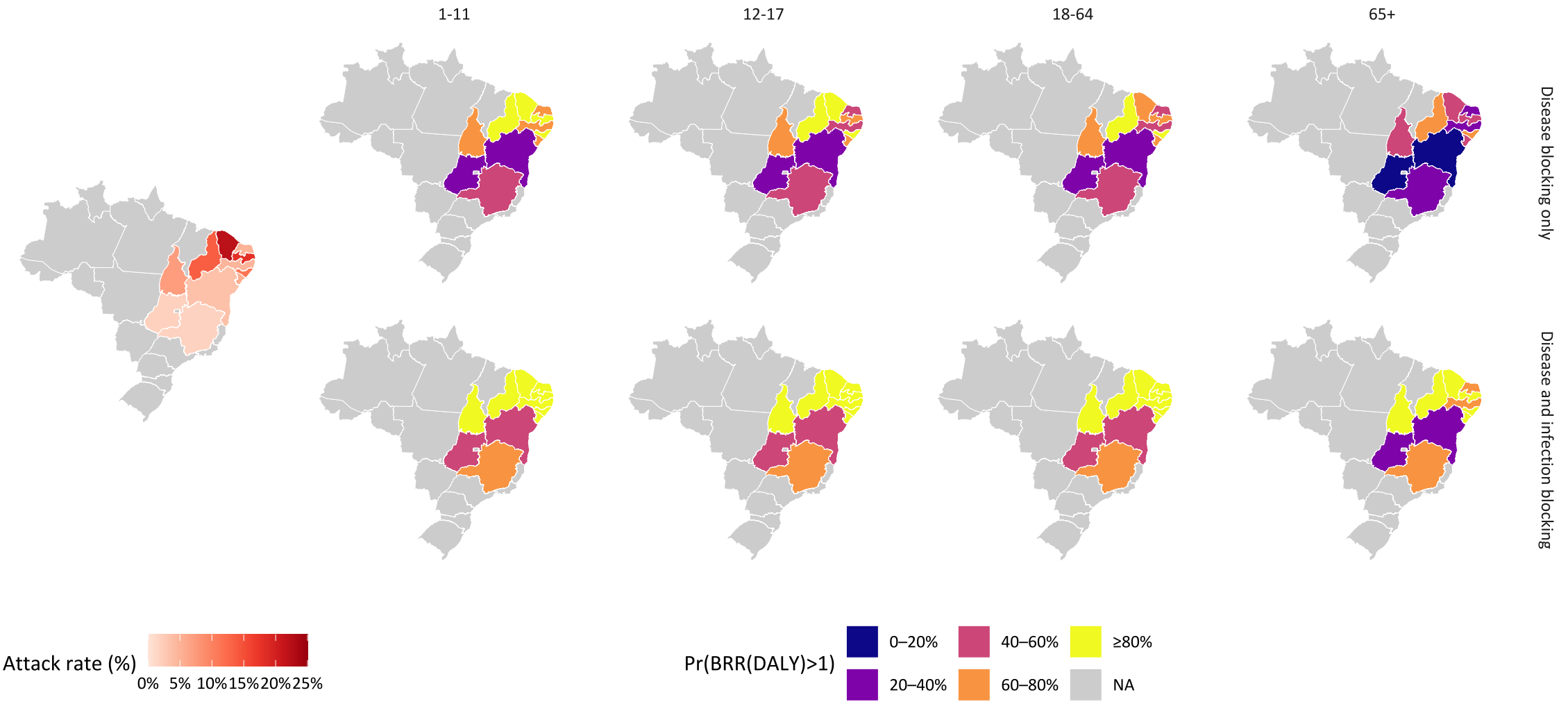
Benefit-risk ratio of outbreak response immunisation: \Pr(\text{BRR}(\text{DALY}) > 1) by vaccine protection mechanism and age group
