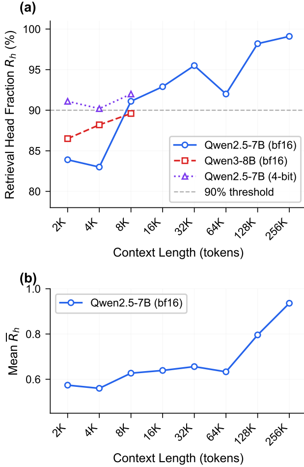
FIG. 6. Retrieval head statistics vs. context length. (a) Retrieval head fraction R_h(\tau=0.3) for Qwen2.5-7B (bf16 and 4-bit) and Qwen3-8B (bf16). The fraction exceeds 90% for n \geq 8K and approaches 99% at 256K context. (b) Mean retrieval ratio \bar{R}_h for Qwen2.5-7B (bf16), showing that individual-head retrieval strength also increases with context length.
