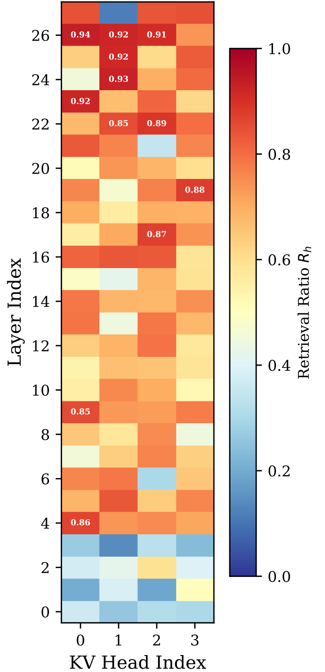
FIG. 5. Retrieval ratio R_h^{(\ell, h)} for each KV head across all layers. Heads with R_h > 0.3 (dashed line) are classified as retrieval heads. (a) Qwen2.5-7B: 102/112 heads are retrieval heads (91.1%) at 8K context. (b) Qwen3-8B: 258/288 heads are retrieval heads (89.6%) at 8K context.
