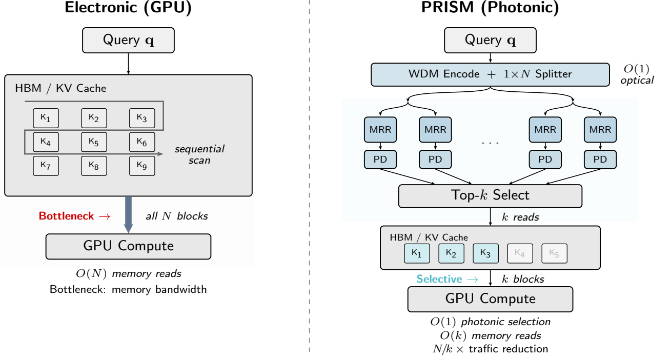
FIG. 1. Conceptual comparison of KV cache access strategies. Left: Electronic GPU full scan—the processor sequentially reads all N KV blocks from HBM to compute attention, bottlenecked by memory bandwidth. Right: PRISM photonic block selection—the query is broadcast optically to all N signature channels in parallel; only the top- k highest-scoring blocks are fetched from memory, reducing traffic by N/k times.
