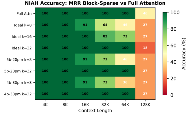
FIG. 8. NIAH accuracy heatmap across context lengths (4K–128K) and MRR configurations. At k=32 , all MRR variants match full attention perfectly up to 64K. Under the k=8 stress test, accuracy degrades gracefully with context length but remains above 90% at 16K. The 128K column shows model-intrinsic degradation (full attention itself drops to 45.5%).
