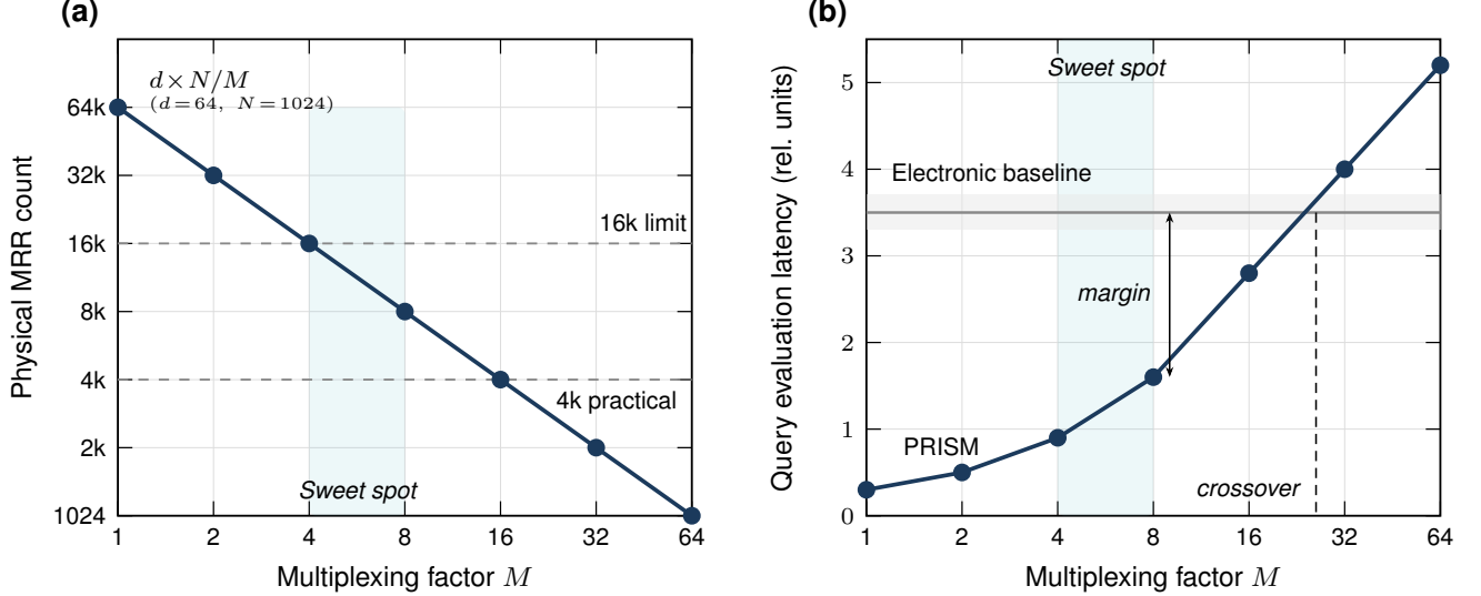
FIG. 10. Time-multiplexed PRISM operation. (a) Physical MRR count vs. multiplexing factor M ( d = 64 , N = 1024 ). (b) Query evaluation latency vs. M , compared to electronic baselines. The shaded region indicates the sweet spot ( M = 4 – 8 ).
