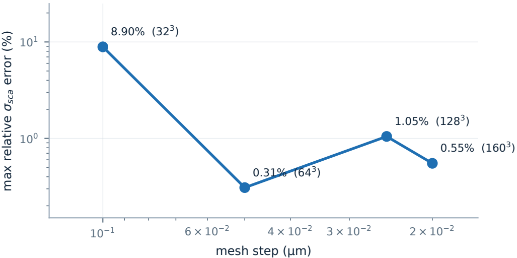
TFSF sphere vs analytic Mie series, 9 wavelengths
