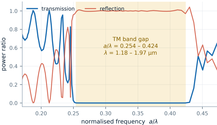
10 rod rows, a = 0.5 \mu\text{m} , r/a = 0.2 , n = 3.4
