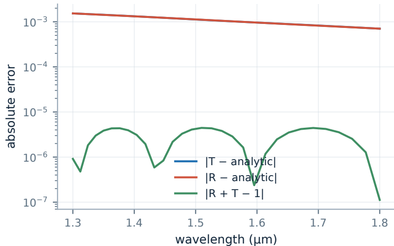
Error against the closed-form solution
