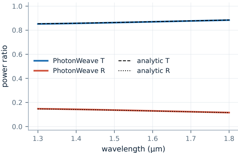
n = 1.5 slab, 0.2 \mu\text{m} thick, 31 frequencies
