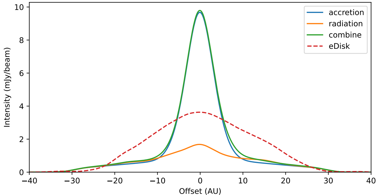
Continuum radial profile along the major axis ( a_{max} = 0.05\text{mm} )
