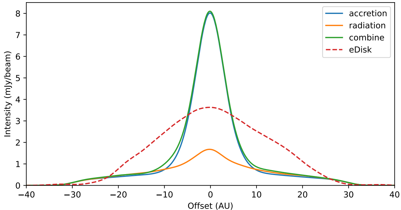
Continuum radial profile along the major axis ( a_{max} = 0.1\text{mm} )
