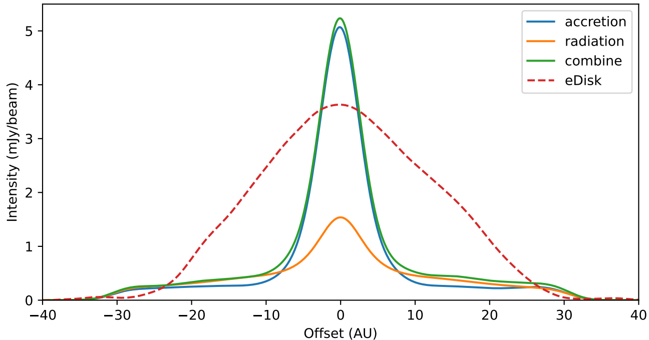
Continuum radial profile along the major axis ( a_{max} = 0.5\text{mm} )
