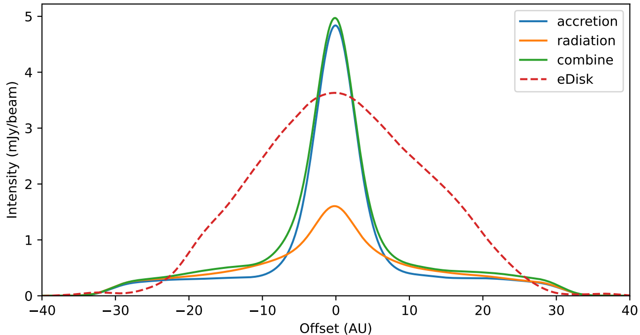
Continuum radial profile along the major axis ( a_{max} = 1.0\text{mm} )
