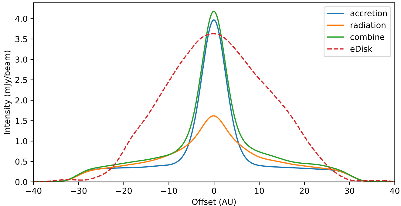
Continuum radial profile along the major axis ( a_{max} = 10.0\text{mm} )
