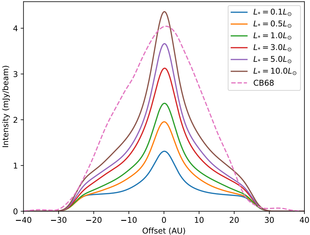
Continuum radial profile along the major axis
