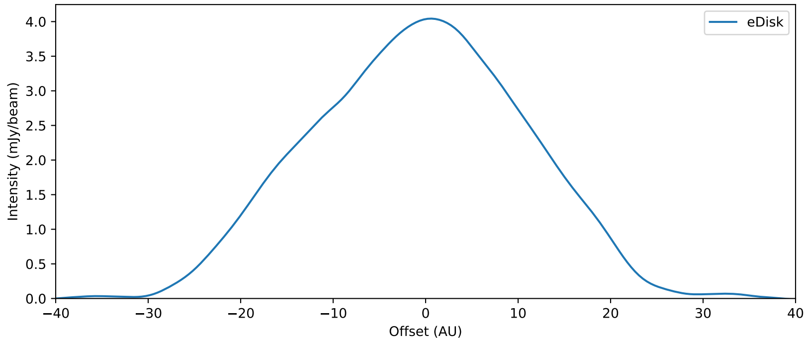
Continuum radial profile along the major axis (eDisk)
