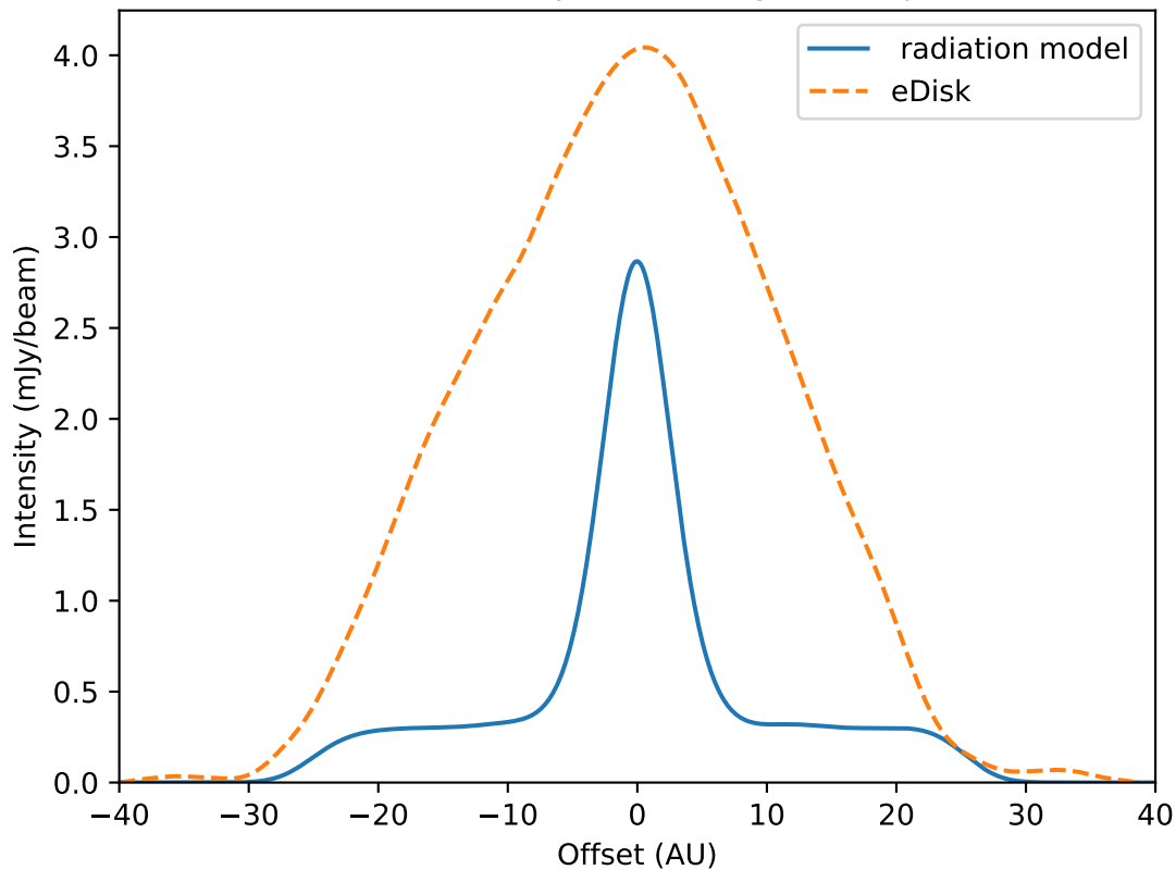
Continuum radial profile along the major axis
