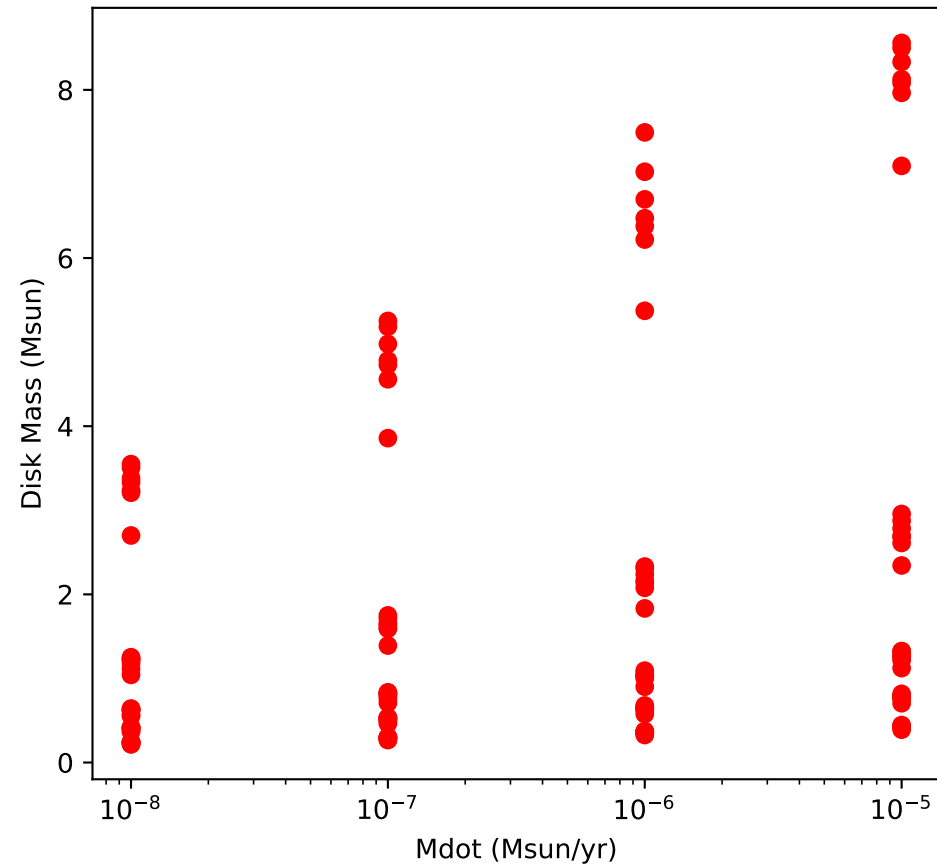
Accretion rate vs. Md
