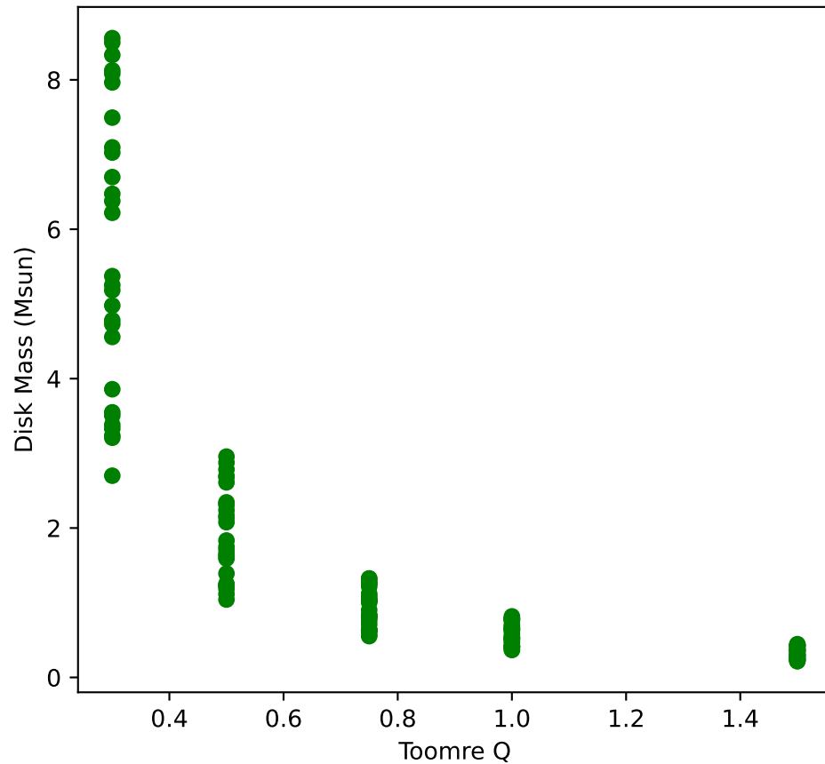
Toomre Q vs. Md
