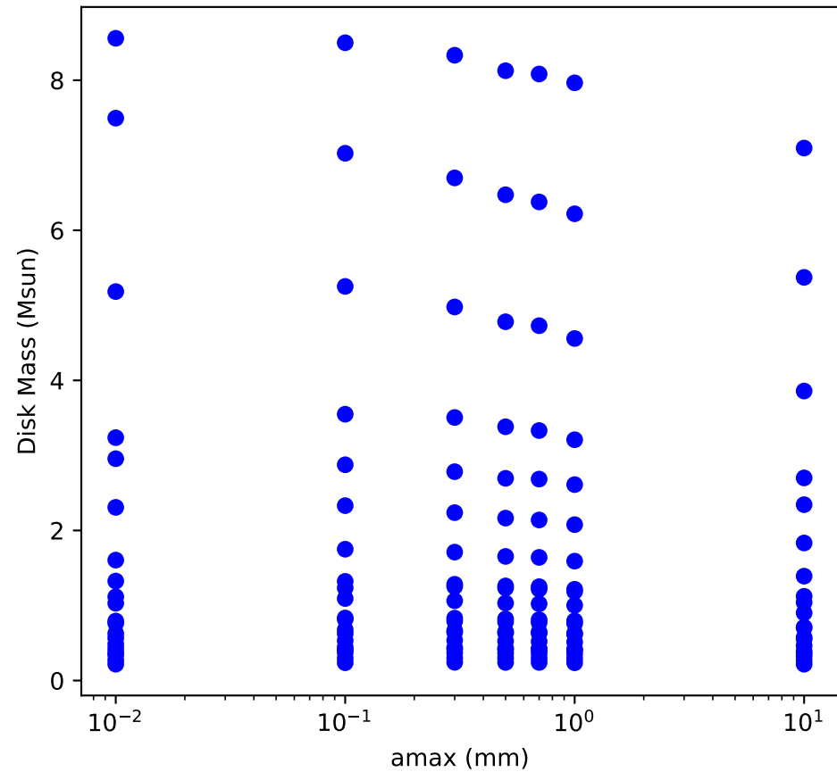
Maximum grain size vs. Md
