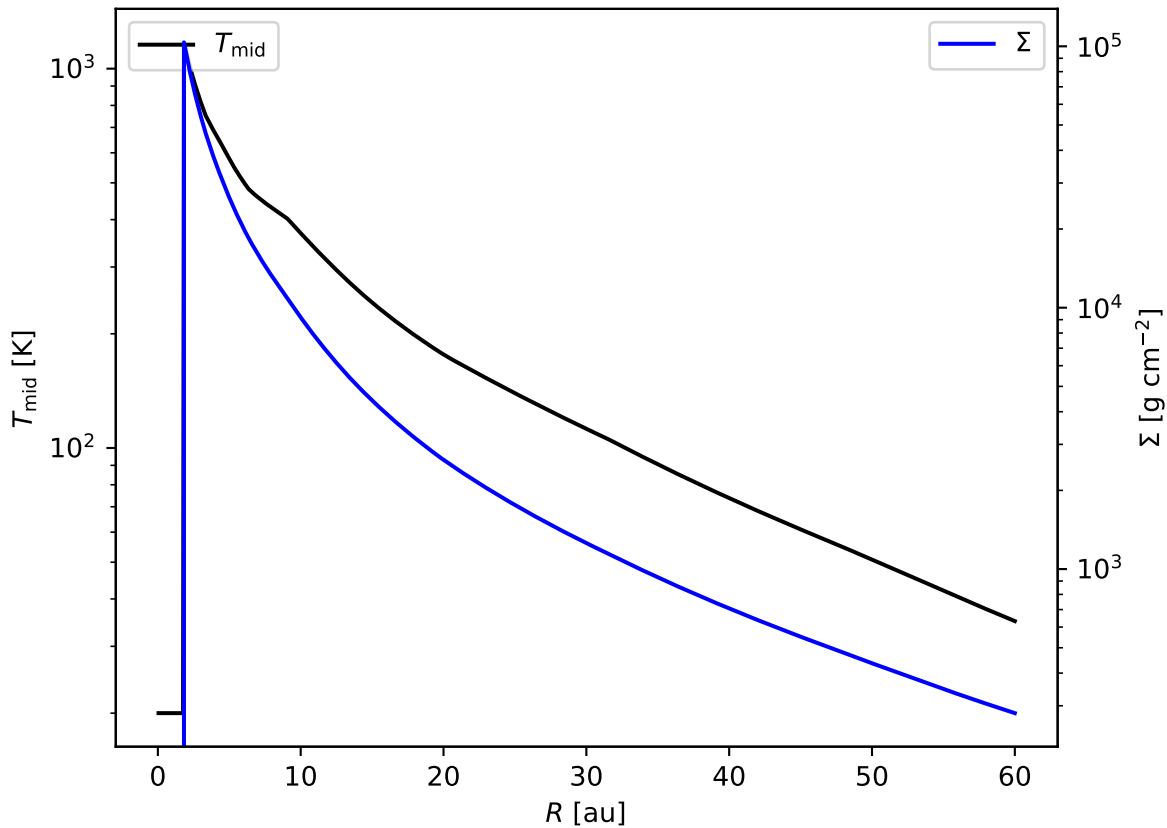
Disk Model: Midplane Temperature and Surface Density
