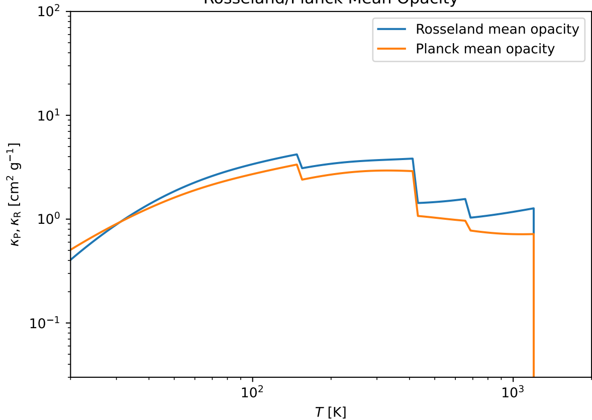
Rosseland/Planck Mean Opacity
