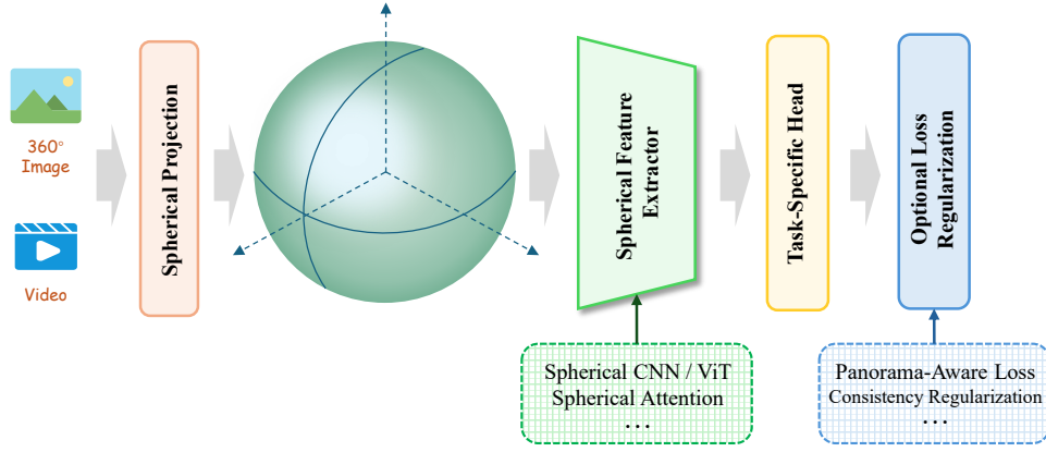
Figure 16 General pipeline for spherical computer vision. The sphere represents the viewing domain of a 360° image or video; individual methods process planar projections or a discrete spherical representation of this domain. A geometry-aware feature extractor and task-specific head produce predictions, with optional panorama-aware losses or consistency regularization during training. The dashed boxes list representative feature extractors and regularizers.
