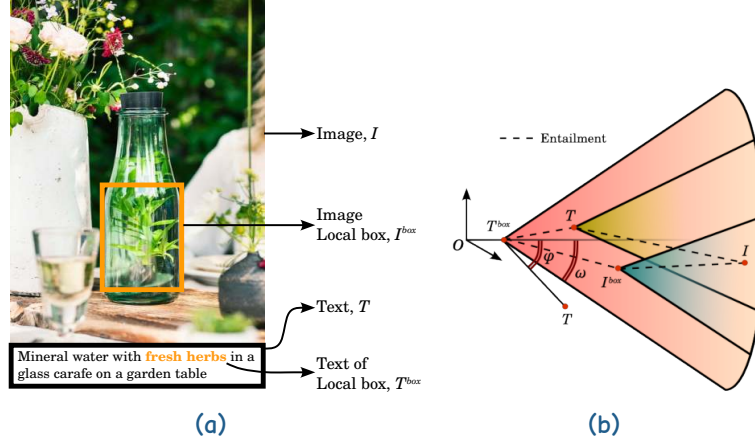
Figure 19 HyCoCLIP compositional entailment [209]. (a) Global pairs (I, T) provide context for local regions (I^{\text{box}}, T^{\text{box}}) . (b) Hyperbolic entailment cones define the desired hierarchical global-local alignment during training.
