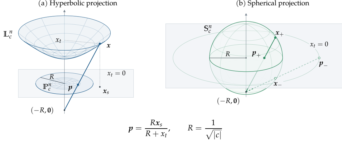
Figure 4 Stereographic projections of the hyperboloid and sphere, shown for n = 2 . Write x = (x_t, x_s)^T , with x_t the vertical coordinate and x_s \in \mathbb{R}^n . Both panels project from (-R, 0) onto the gray plane x_t = 0 using the displayed map. (a) For c < 0 , the Lorentz upper sheet \mathbb{L}_c^n maps onto the Poincaré ball \mathbb{P}_c^n of radius R ; dotted guides mark the coordinates x_t and x_s of x . (b) For c > 0 , upper and lower hemisphere points x_+ and x_- map inside and outside the radius- R equator circle, respectively. The spherical chart covers all of \mathbb{R}^n , with \|p\| \rightarrow \infty as x approaches the excluded south pole.
