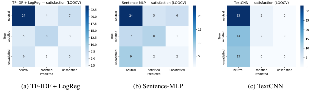
Figure 4: Confusion matrices for satisfaction prediction (3-class, LOOCV n = 64 ).
