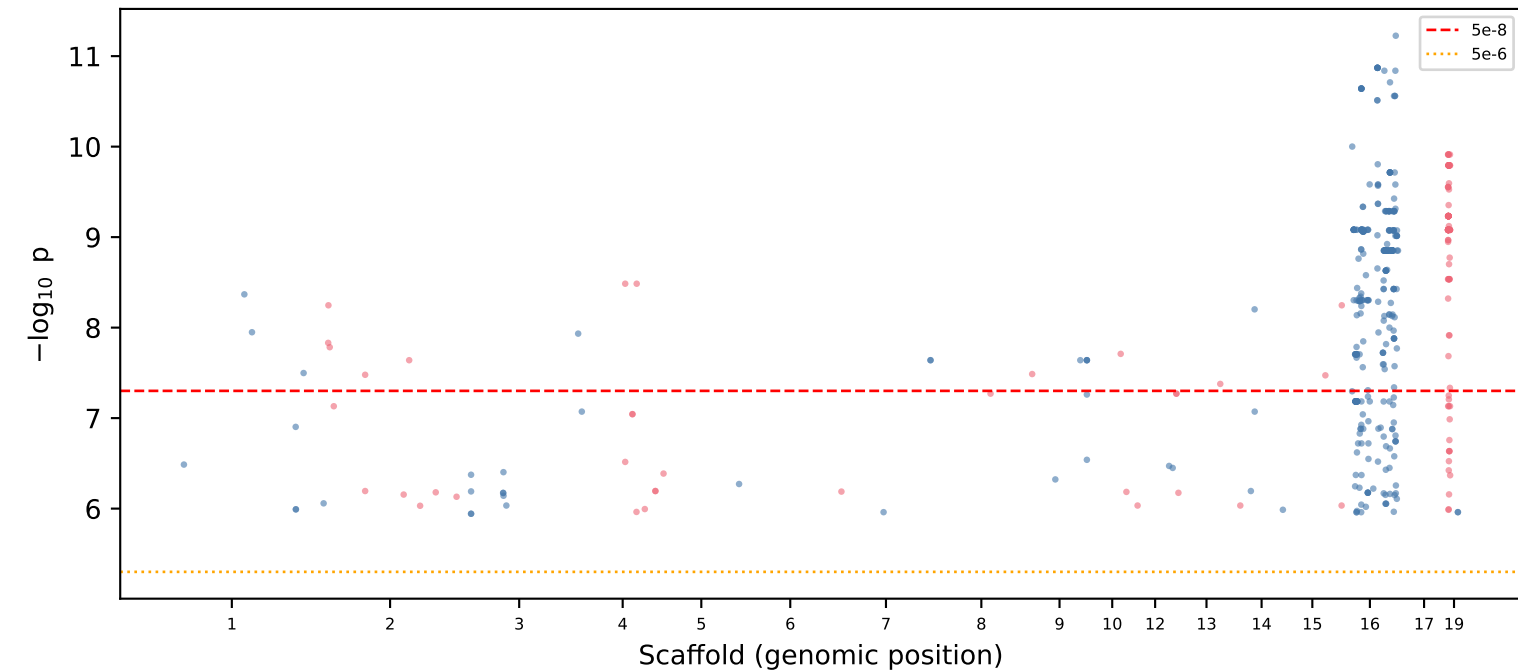
copper multi-Fisher (gwas) top500
