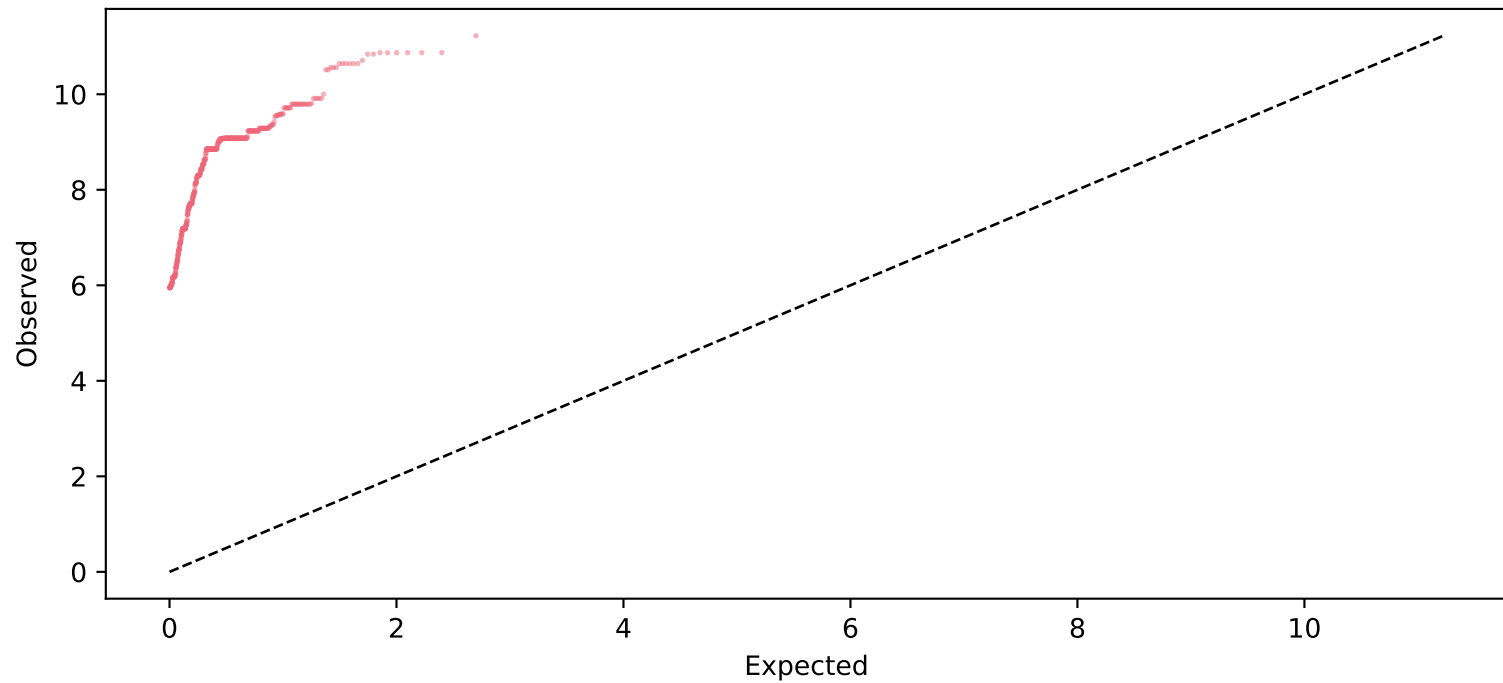
copper multi-Fisher (gwas) top500
