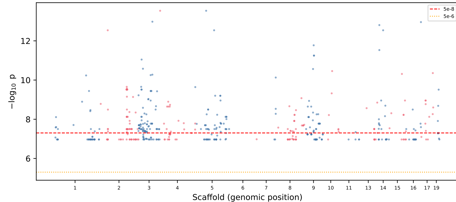
color multi-Fisher (gwasc) top500
