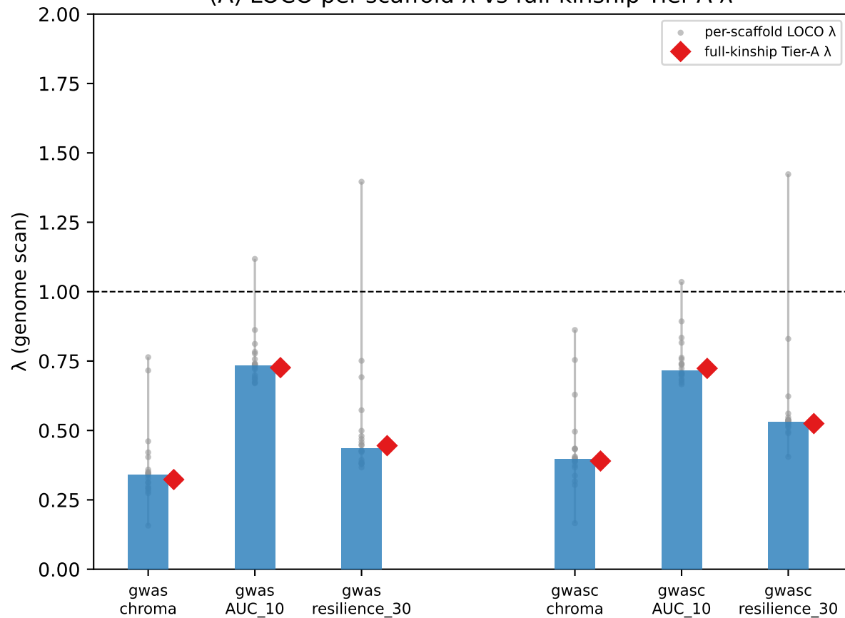
(A) LOCO per-scaffold \lambda vs full-kinship Tier-A \lambda
