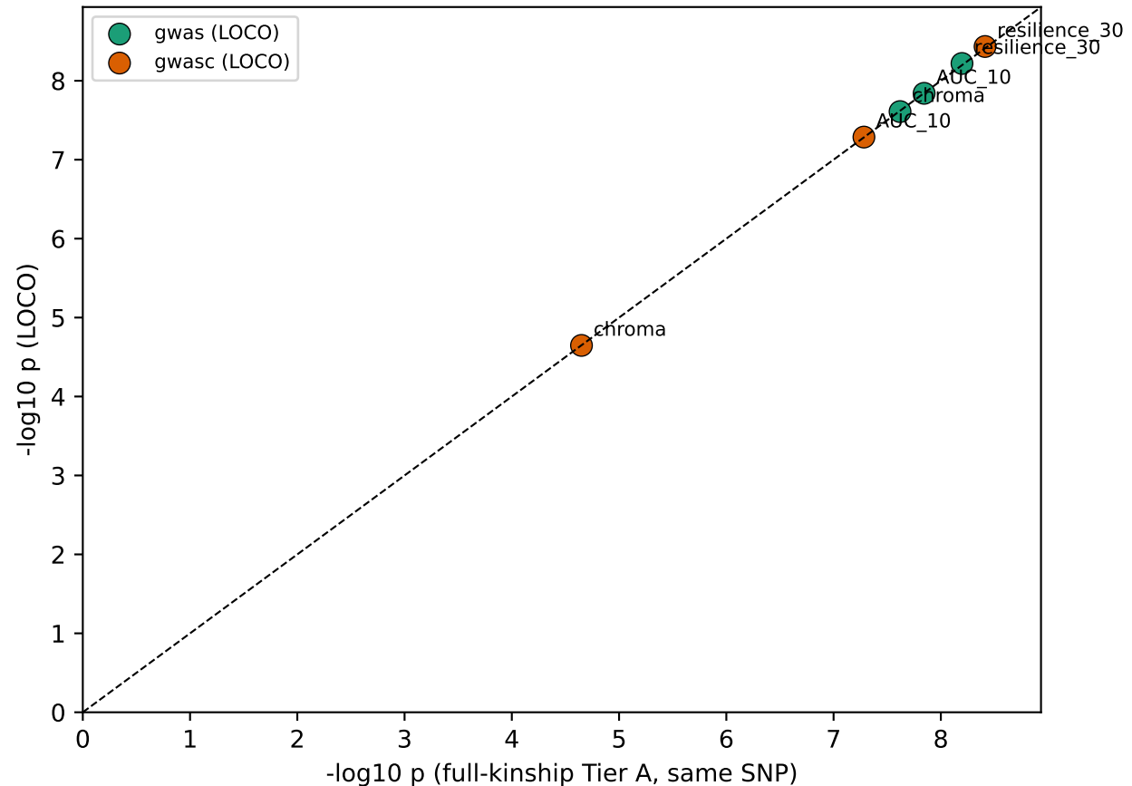
(B) anchor loci: LOCO vs Tier-A same-SNP
