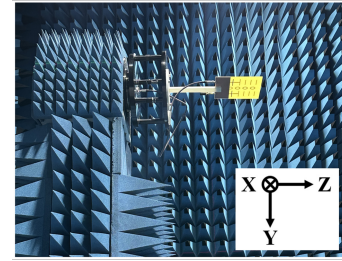
Fig. 11. The antenna measurement setup in the anechoic chamber.
