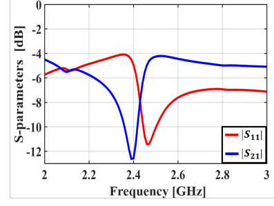
Fig. 8. Frequency response of the designed SRR: |S_{11}| & |S_{21}| .
