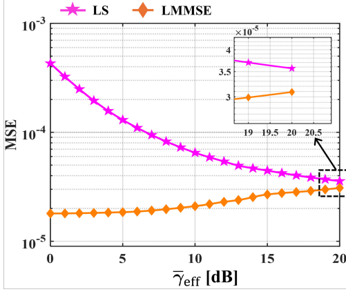
Fig. 27. MSE of the lifted LS and LMMSE estimators over varying \bar{\gamma}_{\text{eff}} .
