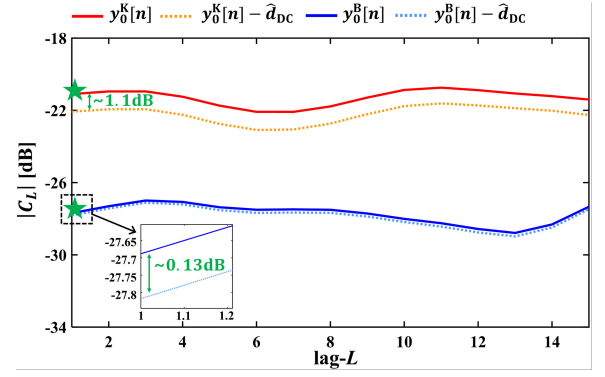
Fig. 18. Validation of the lag-1 uncorrelated-sample assumption for the CFO estimator under the adopted pulse shaping and sampling. The markers indicate the lag-1 value |C_1| .
