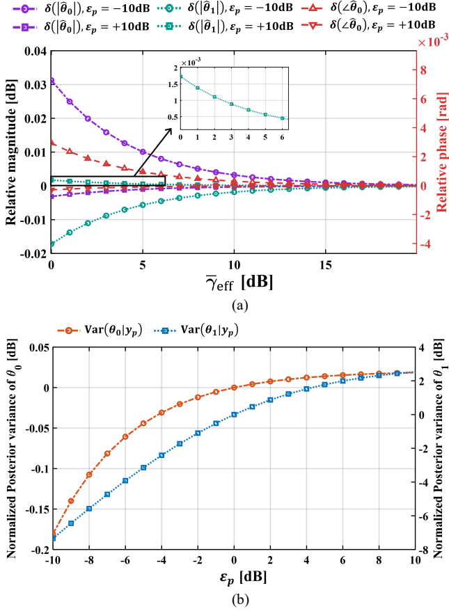
Fig. 30. Sensitivity of the lifted LMMSE estimator to diagonal prior variance mis-specification: (a) relative deviations of the estimated coefficients and phase angle versus \bar{\gamma}_{\text{eff}} , and (b) normalized posterior variances in dB versus \epsilon_p .
