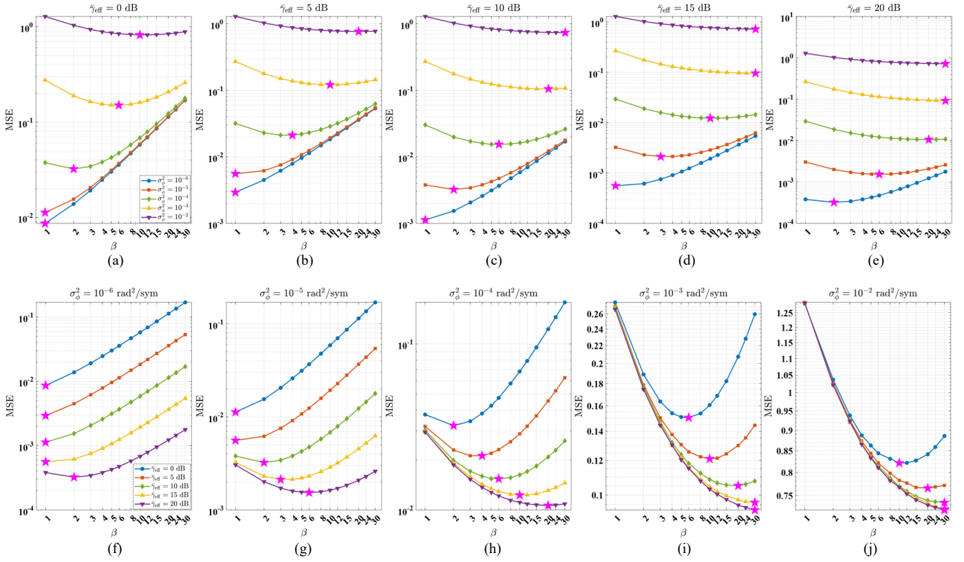
Fig. 25. MSE versus pilot dispersion parameter \beta under varying per-symbol phase drift variance \sigma_\phi^2 and \tilde{\gamma}_{\text{eff}} : (a) \tilde{\gamma}_{\text{eff}} = 0 dB, (b) \tilde{\gamma}_{\text{eff}} = 5 dB, (c) \tilde{\gamma}_{\text{eff}} = 10 dB, (d) \tilde{\gamma}_{\text{eff}} = 15 dB, (e) \tilde{\gamma}_{\text{eff}} = 20 dB, (f) \sigma_\phi^2 = 10^{-6} rad 2 /sym, (g) \sigma_\phi^2 = 10^{-5} rad 2 /sym, (h) \sigma_\phi^2 = 10^{-4} rad 2 /sym, (i) \sigma_\phi^2 = 10^{-3} rad 2 /sym, and (j) \sigma_\phi^2 = 10^{-2} rad 2 /sym.
