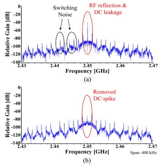
Fig. 13. Frequency spectrum of the receiver during data reception at the center frequency of 2.45 GHz: (a) before and (b) after DC offset removal.
