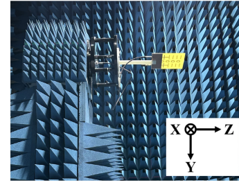
Fig. 11. Antenna measurement setup in the anechoic chamber.
