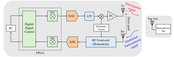
Fig. 12. Block diagram of the SDR reader implementing preprocessing through digital signal control on the FPGA.
