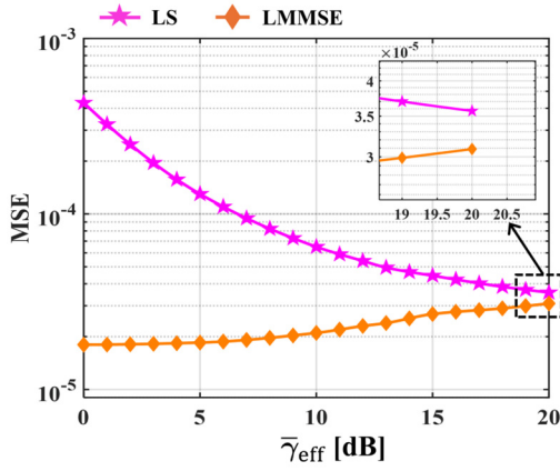
Fig. 27. MSE of the lifted LS and LMMSE estimators over varying \bar{\gamma}_{eff} .
