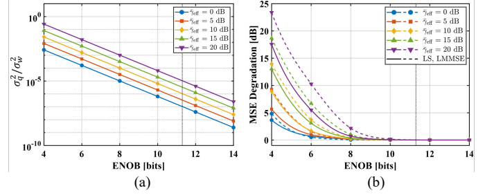
Fig. 15. Impact of ADC resolution on CE performance across \tilde{\gamma}_{\text{eff}} : (a) quantization-to-thermal noise power ratio \sigma_q^2/\sigma_w^2 versus ENOB, and (b) MSE degradation of the lifted LS and LMMSE estimators relative to the infinite-precision baseline versus ENOB. The vertical dotted line indicates the measured operating ENOB of the deployed ADC.
