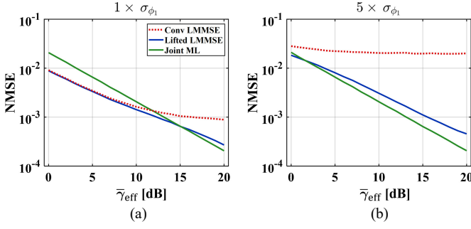
Fig. 32. CE NMSE of the conventional LMMSE, lifted LMMSE, and joint ML (without linearization) estimators: (a) measured operating drift and (b) 5 \times drift stress condition.
