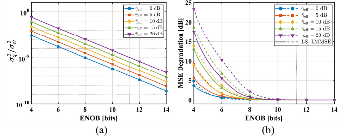
Fig. 15. Impact of ADC resolution on CE performance across \gamma_{\text{eff}} : (a) quantization-to-thermal noise power ratio \sigma_q^2/\sigma_w^2 versus ENOB, and (b) MSE degradation of the lifted LS and LMMSE estimators relative to the infinite-precision baseline versus ENOB. The vertical dotted line indicates the measured operating ENOB of the deployed ADC.
