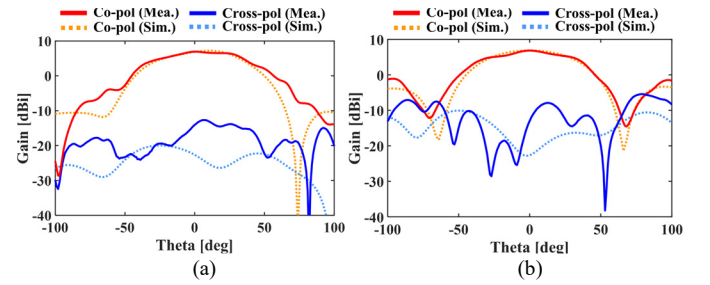
Fig. 10. Simulated and measured gain radiation patterns at 2.45 GHz for (a) \phi = 0^\circ in xz -plane and (b) \phi = 90^\circ in yz -plane.
