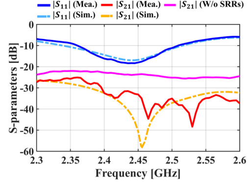
Fig. 9. Simulated and measured S-parameters of the proposed antenna: |S_{11}| & |S_{21}| .
