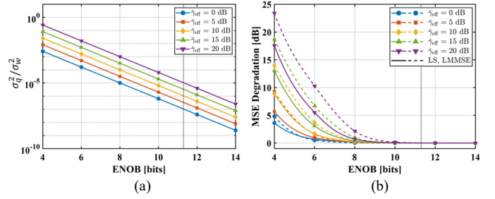
Fig. 15. Impact of ADC resolution on CE performance across \bar{\gamma}_{\text{eff}} : (a) quantization-to-thermal noise power ratio \sigma_q^2/\sigma_w^2 versus ENOB, and (b) MSE degradation of the lifted LS and LMMSE estimators relative to the infinite-precision baseline versus ENOB. The vertical dotted line indicates the measured operating ENOB of the deployed ADC.
