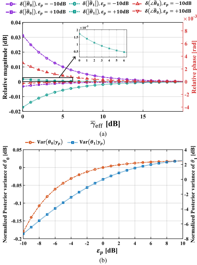
Fig. 30. Sensitivity of the lifted LMMSE estimator to diagonal prior variance mis-specification. (a) Relative deviations of the estimated coefficients and phase angle versus \bar{\gamma}_{eff} and (b) normalized posterior variances in dB versus \epsilon_p .
