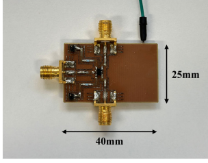
Fig. 4. Designed semi-passive tag for load modulation.
