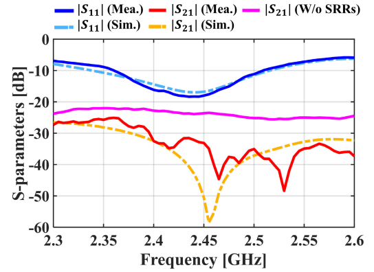
Fig. 9. Simulated and measured S-parameters of the proposed antenna: |S_{11}| and |S_{21}| .
