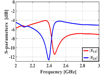
Fig. 8. Frequency response of the designed SRR: |S_{11}| and |S_{21}| .
