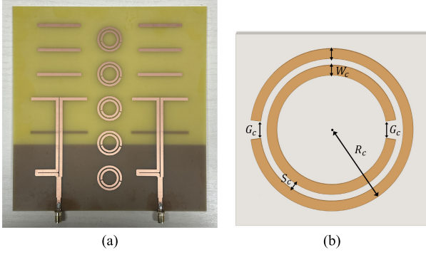
Fig. 6. (a) Fabricated 2 \times 1 planar Yagi-Uda antenna array and (b) geometry of the SRR for isolation improvement.
