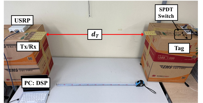
Fig. 16. Indoor experimental setup of the proposed BMC system: d_T = 1 m.
