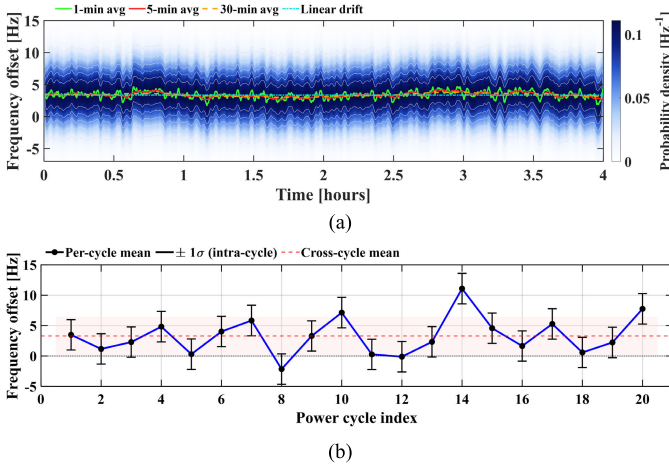
Fig. 22. Temporal stability of the measured frequency offset. (a) 4-h time series showing per-frame \hat{\Delta f} with 1-, 5-, and 30-min moving averages and a linear drift fit, and (b) power-cycle dependence of \hat{\Delta f} showing per-cycle mean with intra-cycle \pm 1\sigma error bars, the cross-cycle mean, and a shaded band indicating cross-cycle mean \pm 1\sigma .
