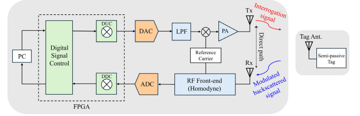
Fig. 12. Block diagram of the SDR reader implementing preprocessing through digital signal control on the FPGA.
