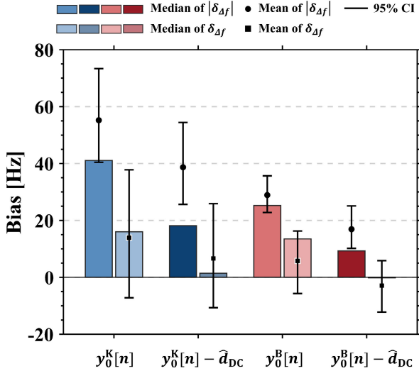
Fig. 19. Signed and absolute bias of the proposed CFO estimator for nonzero-mean OOK pilots and zero-mean BPSK pilots, with 95% confidence intervals (CIs).
