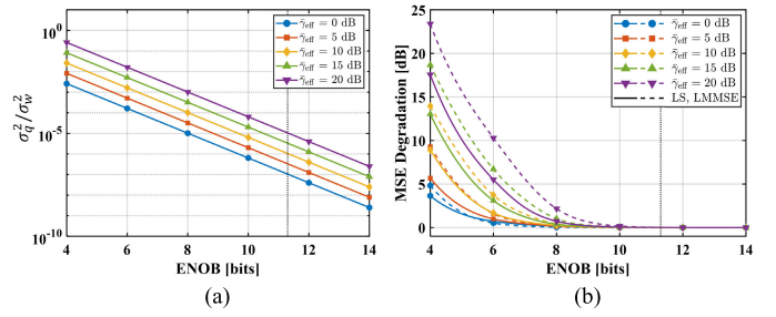
Fig. 15. Impact of ADC resolution on CE performance across \bar{\gamma}_{\text{eff}} : (a) quantization-to-thermal noise power ratio \sigma_q^2/\sigma_w^2 versus ENOB and (b) mse degradation of the lifted LS and LMMSE estimators relative to the infinite-precision baseline versus ENOB. The vertical dotted line indicates the measured operating ENOB of the deployed ADC.
