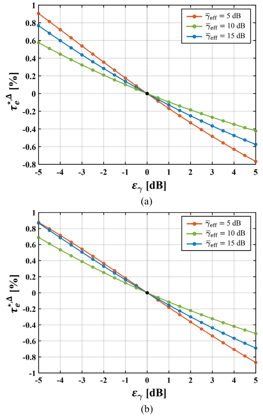
Fig. 23. Optimal pilot duration shifts \tau_e^{*,\Delta} versus SNR estimation error \varepsilon_\gamma , evaluated at \bar{\gamma}_{\text{eff}} \in \{5, 10, 15\} dB. (a) OOK and (b) BPSK.
