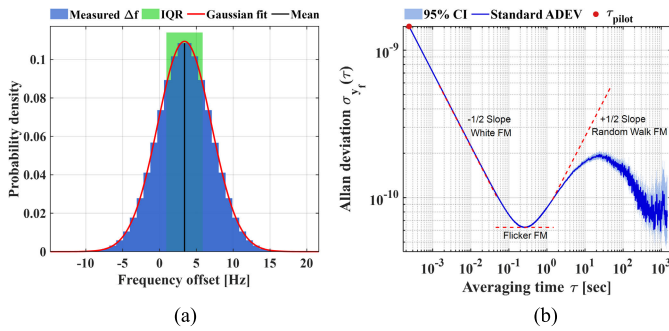
Fig. 21. Statistical characterization of the CFO estimation under a shared reference clock with independent PLLs. (a) Probability density of \Delta f with interquartile range (IQR) shading and (b) Allan deviation of the fractional-frequency fluctuation.
