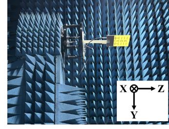
Fig. 11. Antenna measurement setup in the anechoic chamber.
