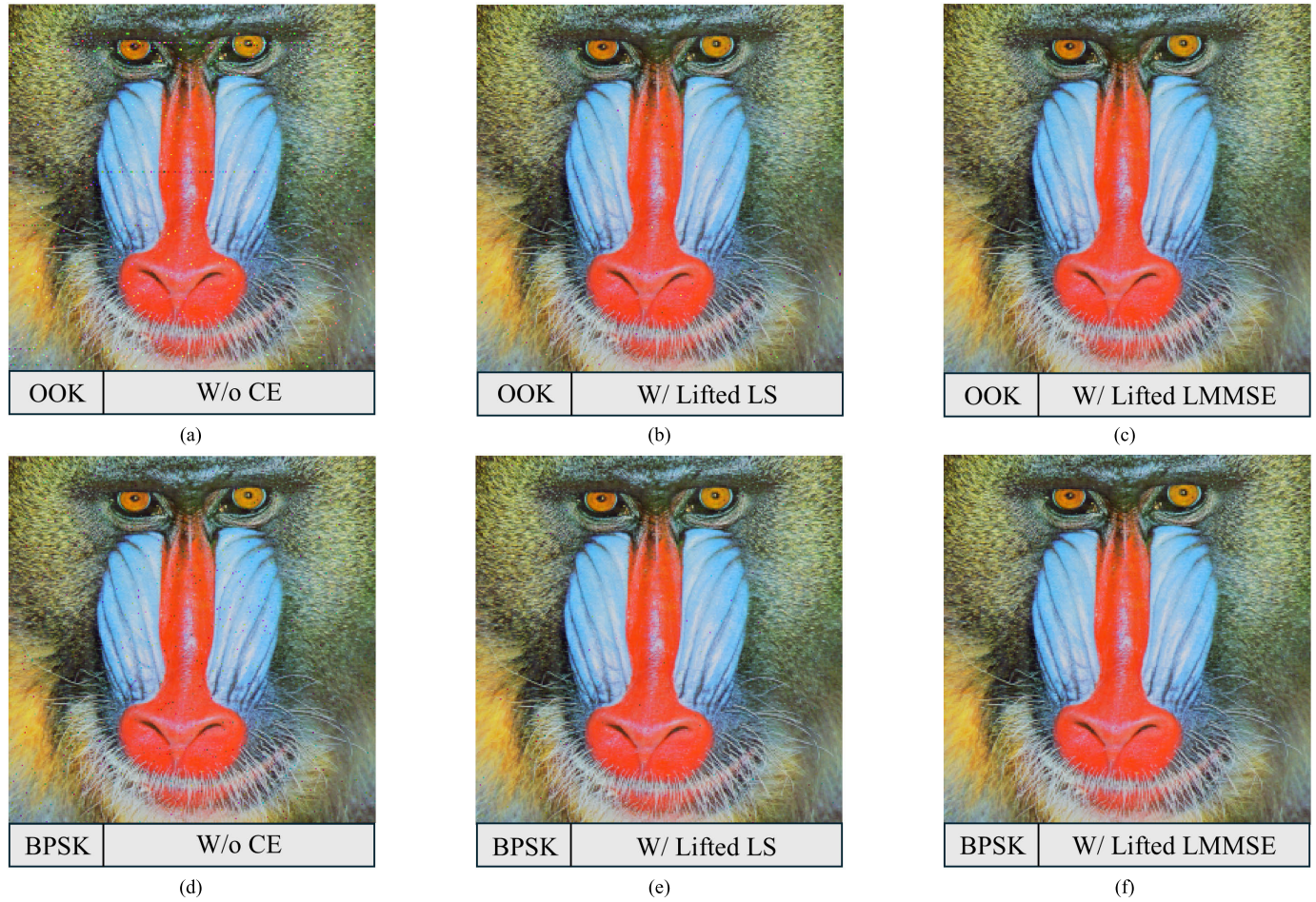
Fig. 36. OTA IR at a fixed operating point, \bar{\gamma}_{\text{eff}} = 15 dB, showing the quantitative impact of CE on end-to-end reliability. (a) OOK without CE at \text{BER} = 9.3 \times 10^{-4} , (b) OOK with the lifted LS at \text{BER} = 5.1 \times 10^{-5} , (c) OOK with the lifted LMMSE at \text{BER} < 10^{-9} , (d) BPSK without CE at \text{BER} = 9.1 \times 10^{-5} , (e) BPSK with the lifted LS at \text{BER} = 1.4 \times 10^{-6} , and (f) BPSK with the lifted LMMSE at \text{BER} < 10^{-9} .
