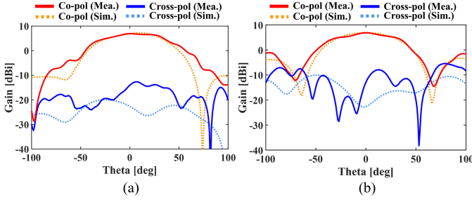
Fig. 10. Simulated and measured gain radiation patterns at 2.45 GHz for (a) \phi = 0^\circ in xz plane and (b) \phi = 90^\circ in yz plane.
