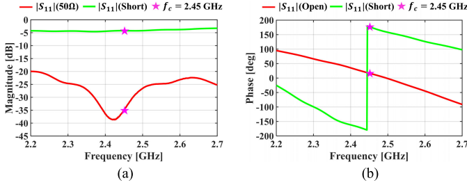
Fig. 5. Measured |S_{11}| of the proposed load modulator (semi-passive tag). (a) Magnitude and (b) phase.
