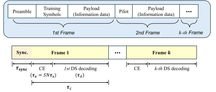
Fig. 2. Frame structure for CE and ID.
