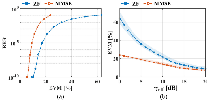
Fig. 34. Noise-enhancement penalty of ZF versus EA MMSE equalization using the estimated \text{Var}(\hat{h}) . (a) BER-EVM characteristic and (b) EVM performance where shaded area denotes the 90% CI propagated from the closed-form posterior covariance.
