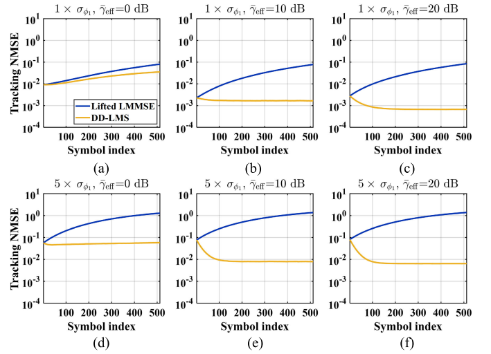
Fig. 33. Data-phase channel tracking NMSE versus symbol index for the pilot-only lifted LMMSE estimate and the DD-LMS adaptive tracker, at \bar{\gamma}_{\text{eff}} \in \{0, 10, 20\} dB: (a)–(c) Measured operating drift and (d)–(f) 5\times drift stress.
