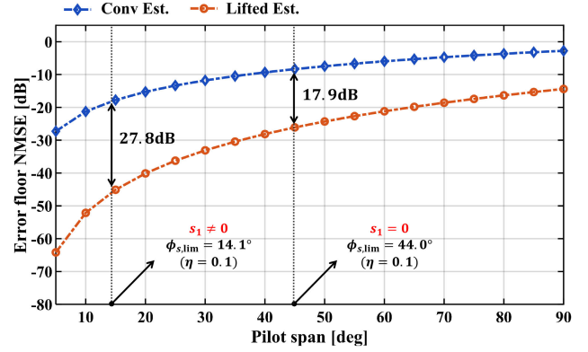
Fig. 29. NMSE floor versus pilot phase span \phi_s for the conventional scalar and lifted estimators. Vertical lines indicate the admissible pilot phase span at \eta = 0.1 for noncentered ( s_1 \neq 0 ) and centered pilot placement ( s_1 = 0 ).
