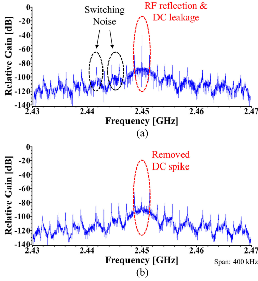
Fig. 13. Frequency spectrum of the receiver during data reception at the center frequency of 2.45 GHz. (a) Before and (b) after DC offset removal.
