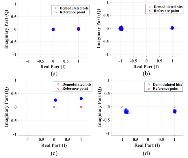
Fig. 17. Constellation diagram after the signal processing chain for OOK and BPSK with and without integrated SRRs. (a) OOK with SRRs, (b) BPSK with SRRs, (c) OOK without SRRs, and (d) BPSK without SRRs.
