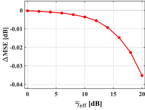
Fig. 28. Matched-SNR CE-MSE difference of the lifted estimator with and without SRRs.
