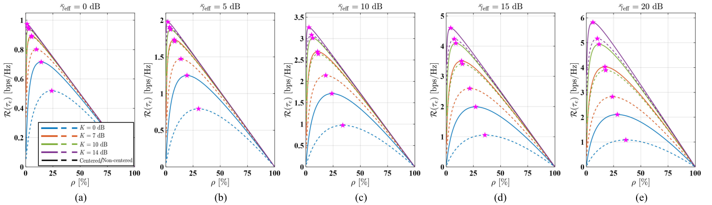
Fig. 26. Spectral efficiency \mathcal{R}(\tau_e) versus pilot overhead \rho for the joint (h_{eq}, \phi_1) estimation framework, evaluated across Rician K -factors at a given \bar{\gamma}_{\text{eff}} . (a) \bar{\gamma}_{\text{eff}} = 0 dB, (b) \bar{\gamma}_{\text{eff}} = 5 dB, (c) \bar{\gamma}_{\text{eff}} = 10 dB, (d) \bar{\gamma}_{\text{eff}} = 15 dB, and (e) \bar{\gamma}_{\text{eff}} = 20 dB.
