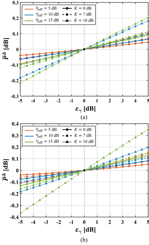
Fig. 24. Sensitivity of BER variation \bar{P}^\Delta versus SNR estimation error \epsilon_\gamma , evaluated at \bar{\gamma}_{\text{eff}} \in \{5, 10, 15\} dB and K \in \{0, 7, 10\} dB. (a) OOK and (b) BPSK.
