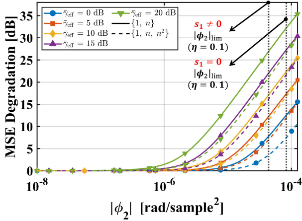
Fig. 3. MSE degradation of the two-parameter ( \{1, n\} ) and three-parameter ( \{1, n, n^2\} ) lifted estimators as a function of the unmodeled quadratic phase coefficient |\phi_2| . The vertical dotted lines indicate the admissible bounds, |\phi_2|_{\text{lim}} at \eta = 0.1 for centered ( s_1 = 0 ) and noncentered ( s_1 \neq 0 ) pilot placement.
