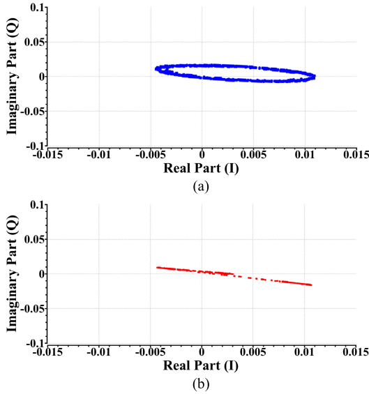
Fig. 14. Constellation diagram of the received data. (a) Before and (b) after CFO compensation for enabling coherent detection.
