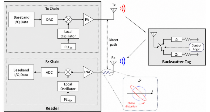
Fig. 1. The phase distortion issue in monostatic backscatter communications.
