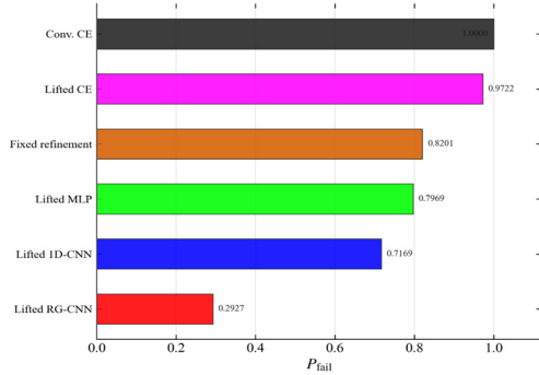
Fig. 7. Tail-failure probability comparison under large residual phase drift, where P_{\text{fail}} = \Pr[\text{NMSE} > -20 \text{ dB}] .
