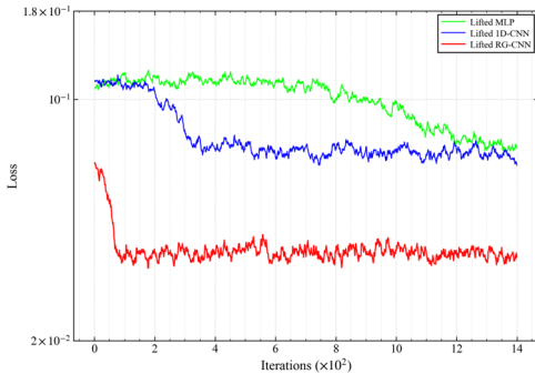
Fig. 3. Training loss convergence.
