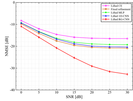
Fig. 4. CE NMSE versus SNR under residual phase drift.
