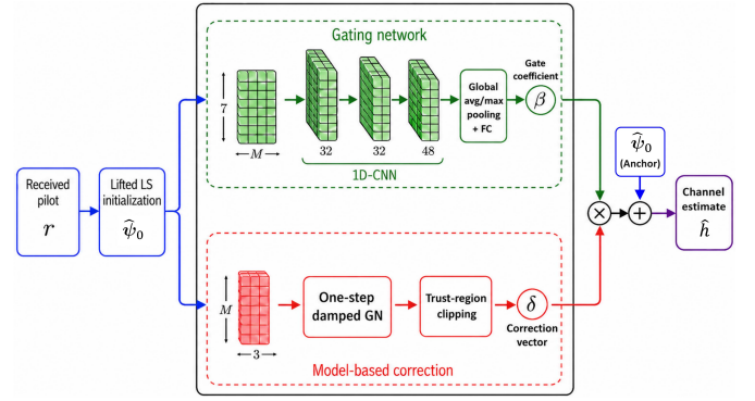
Fig. 2. The proposed RG-CNN architecture for backscatter communication CE.
