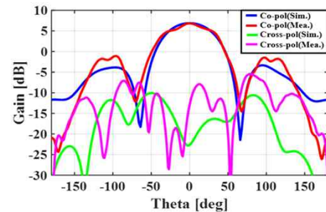
(b) \phi = 90^\circ (yz-평면)
