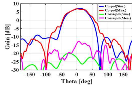
(a) \phi = 0^\circ (xz-평면)
