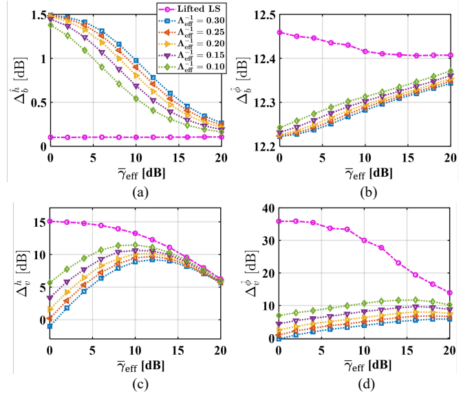
Fig. 31. Bias and variance losses of the lifted estimators relative to the joint ML estimator: bias loss for (a) \hat{h} and (b) \hat{\phi} ; variance loss for (c) \hat{h} and (d) \hat{\phi} . The lifted LS is prior-independent; the lifted LMMSE is parameterized by the prior-to-data precision ratio \Lambda_{\text{eff}}^{-1} .
