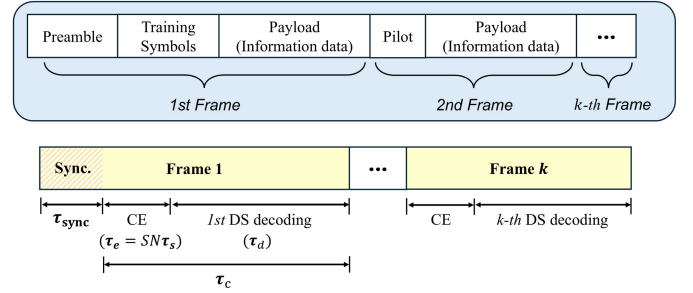
Fig. 2. Frame structure for CE and ID.
