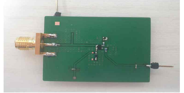
Fig. 4. Fabricated reflection amplifier.
