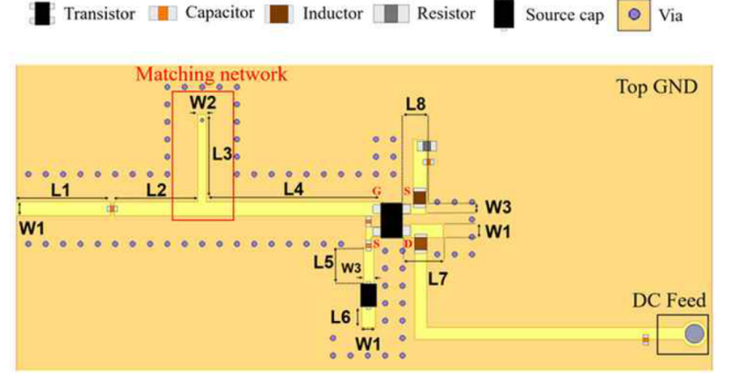
Fig. 3. Reflection-amplifier layout.
