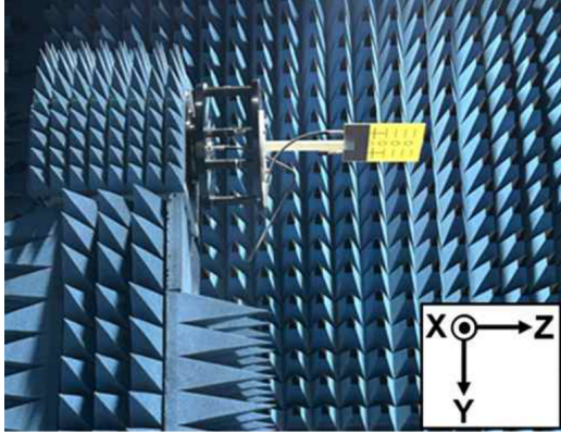
Fig. 10. Antenna measurement environment.
