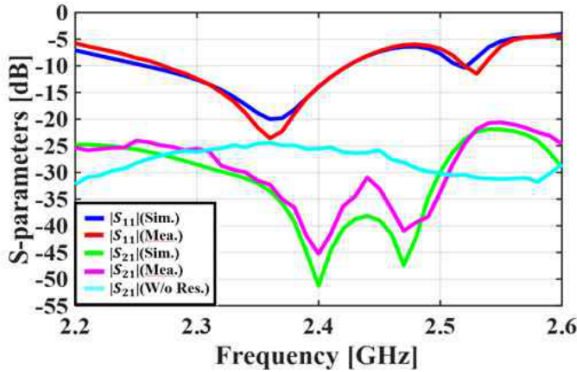
Fig. 11. Measured antenna S-parameters: |S_{11}| and |S_{21}| .
