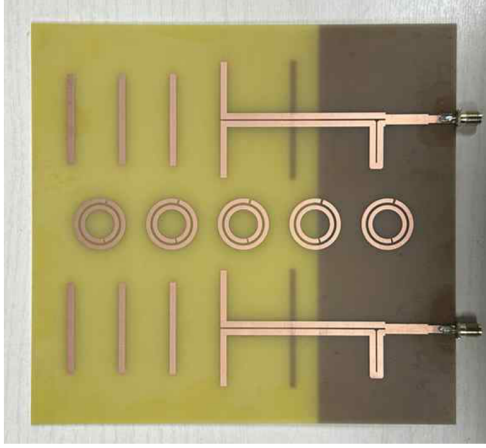
Fig. 7. Proposed 2 \times 1 Yagi-Uda antenna array.
