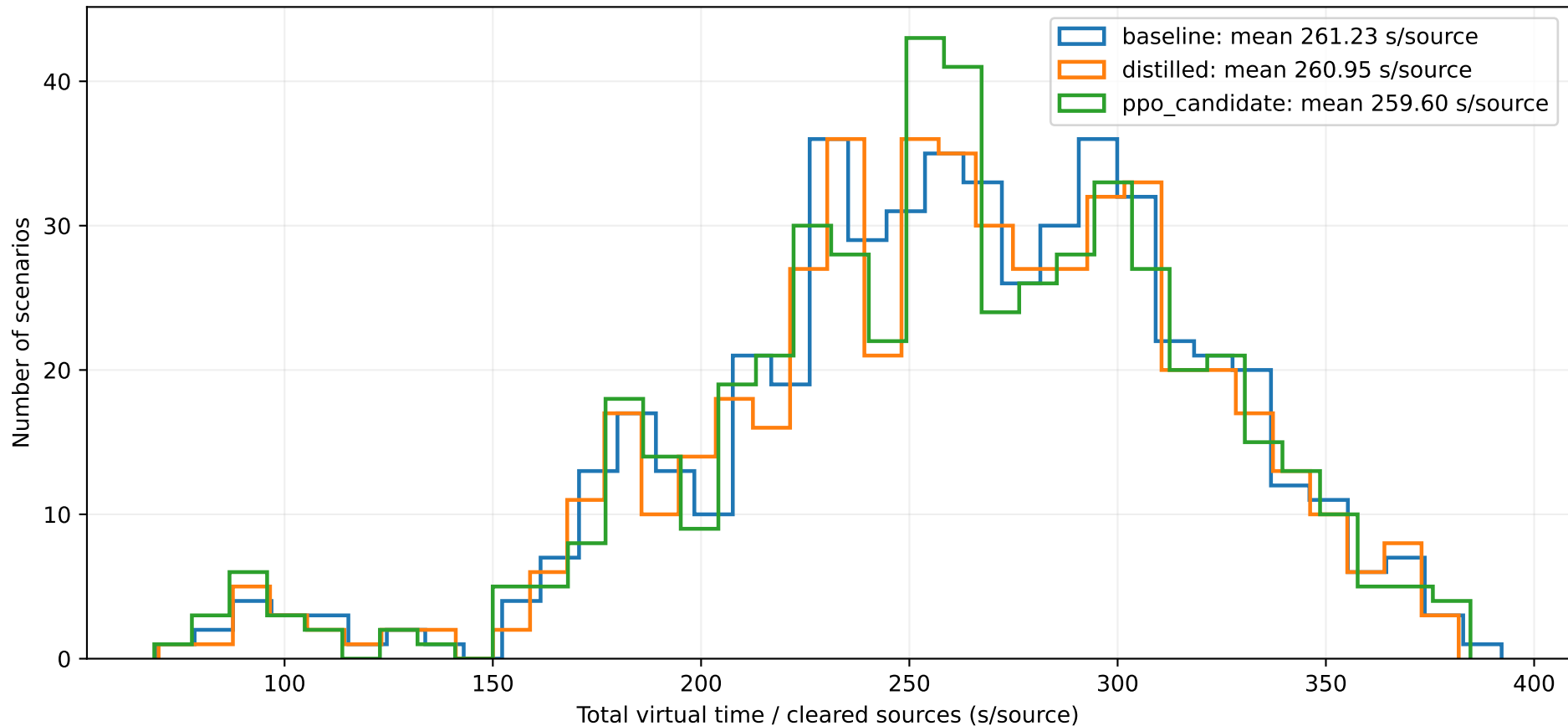
Q3 frozen models: 512 independent LOCAL-RESEARCH scenarios
