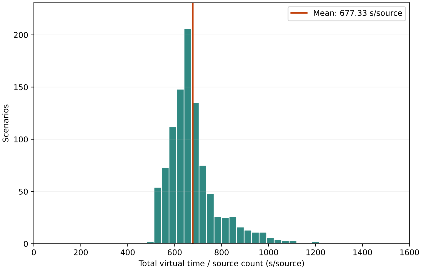
Final Q4 c8812ced | N=15 | 1000/1000 complete
