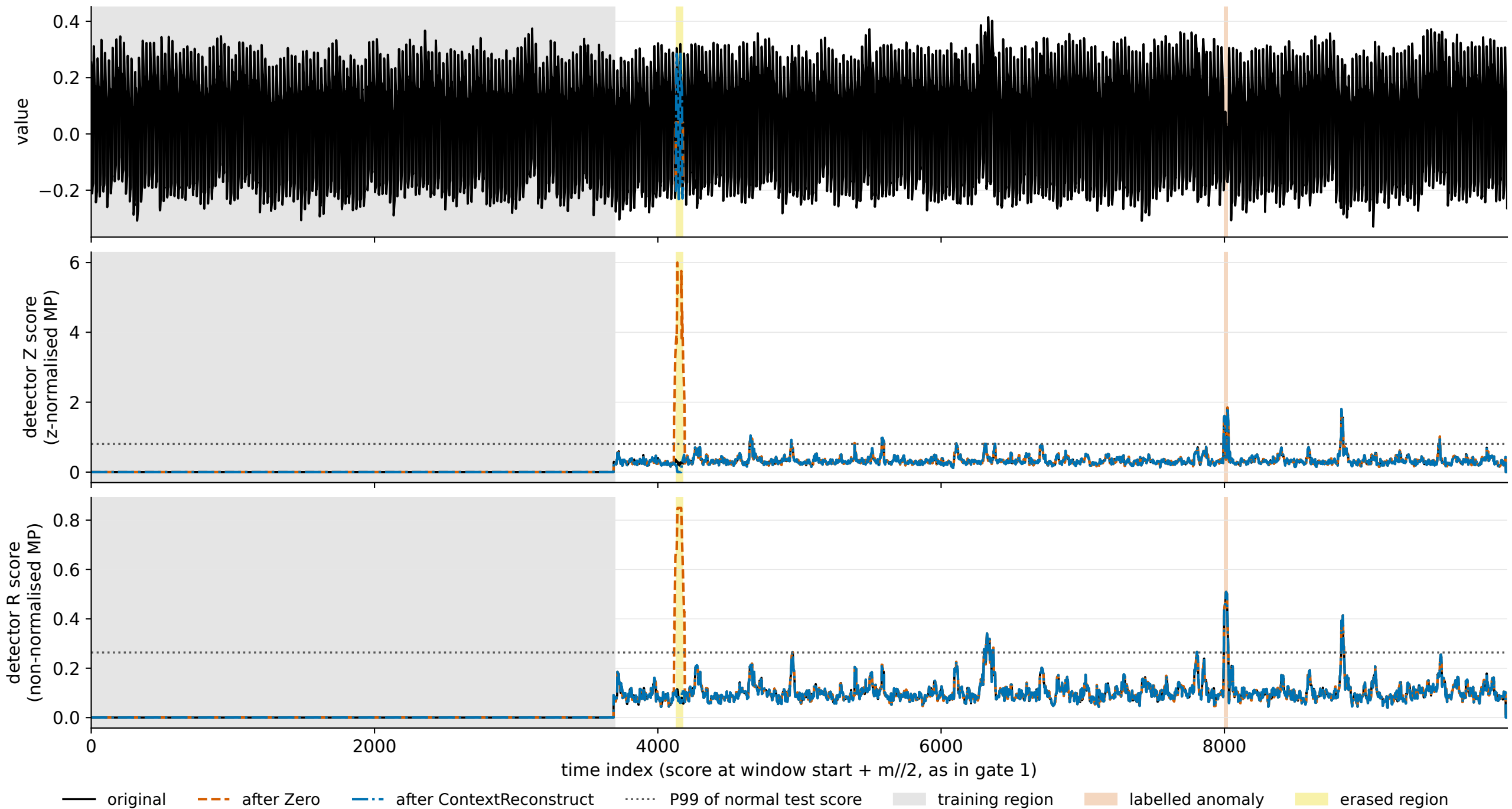
F2 — erasing a normal segment: DISTORTEDinsectEPG2, m = 26 , r = 2m = 52 , erased [4126, 4178) (full series)
