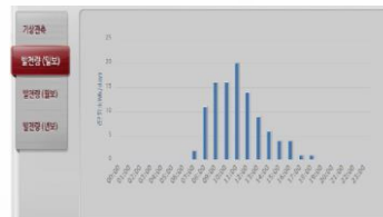
[Generation Graph]
