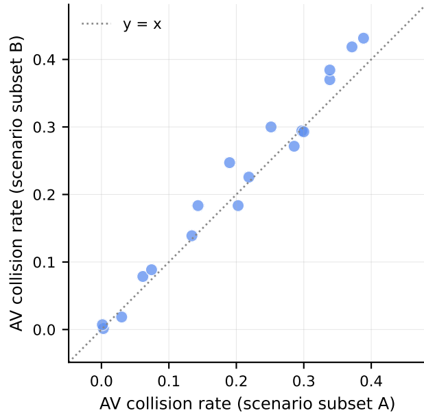
(b) Per-AV collision rate shifts (real grid (AV=18, n_scen=1400))
